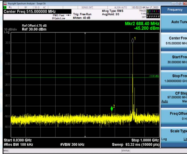
Band26-15MHz-QPSK-26865-1RB#0-Range2:1000~10000MHz
