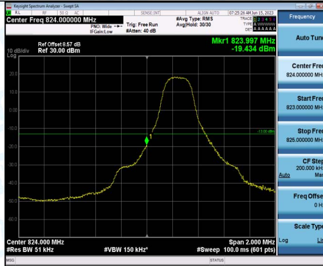
Band26-3MHz-QPSK-26805-1RB#14
