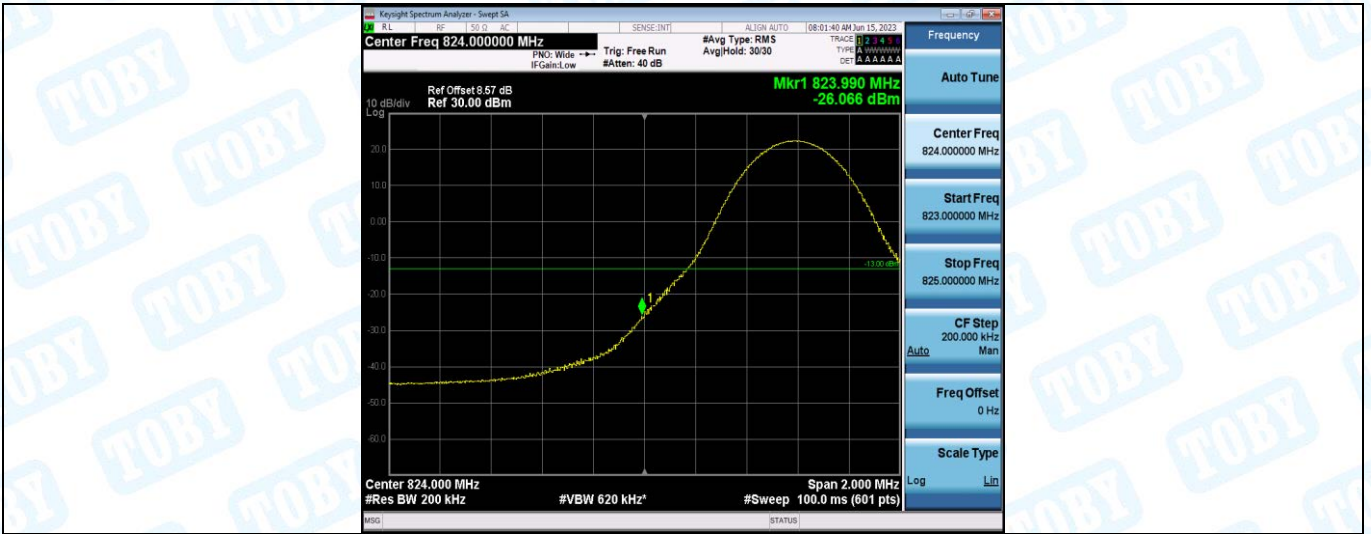
Band26-10MHz-QPSK-26840-1RB#49
