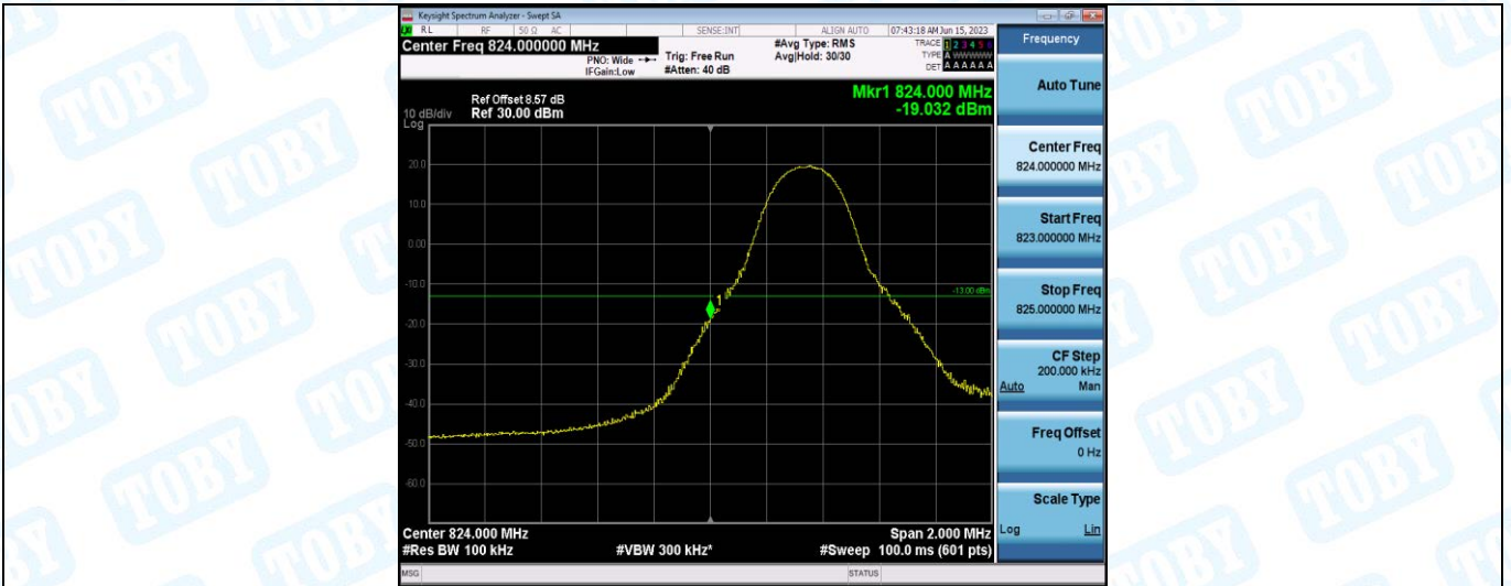
Band26-5MHz-16QAM-26815-1RB#24
