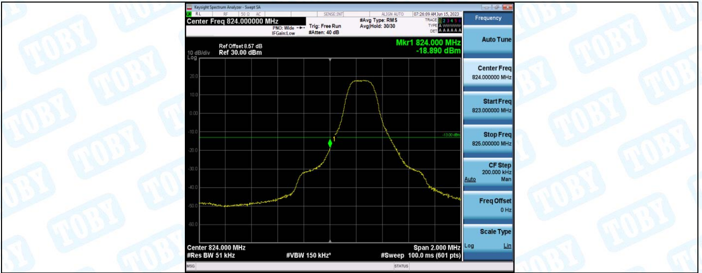
Band26-3MHz-16QAM-26805-1RB#14
