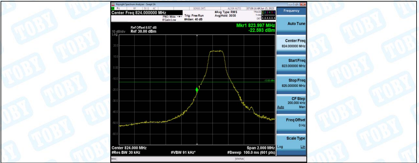
Band26-1.4MHz-16QAM-26797-1RB#5
