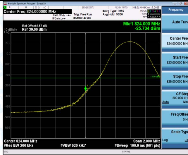
Band26-10MHz-16QAM-26840-1RB#49
