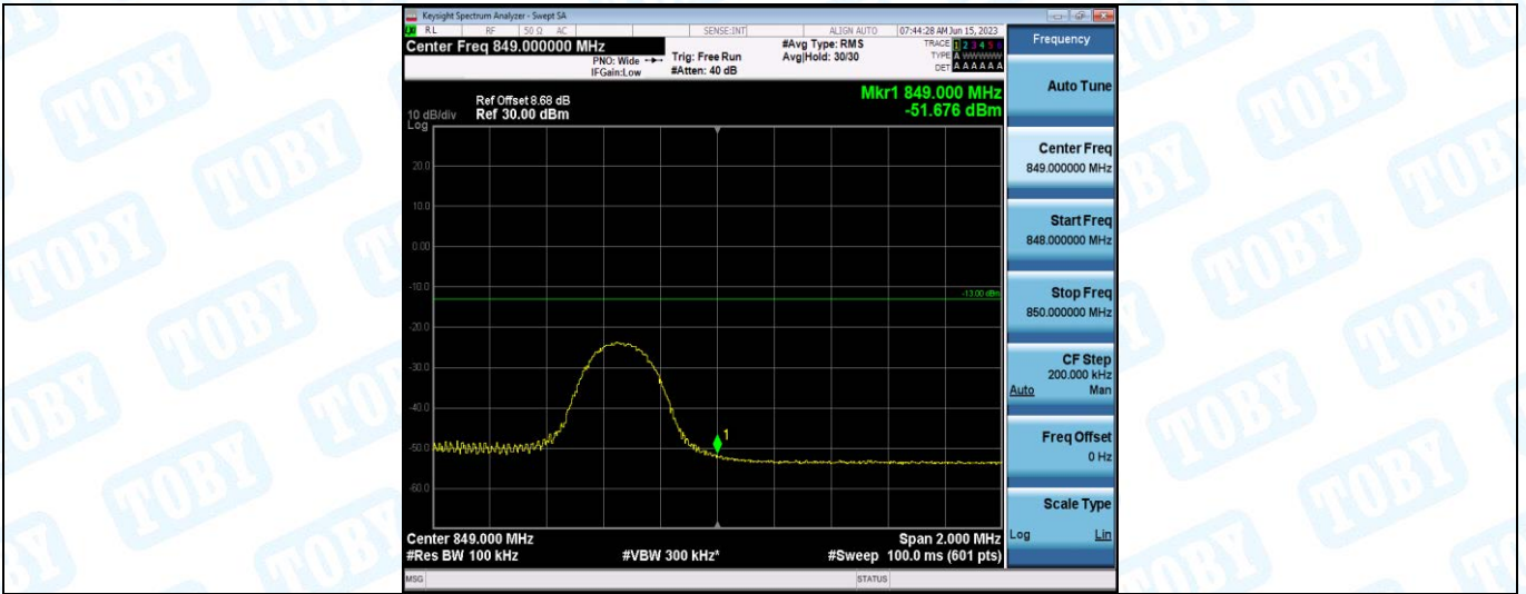
Band26-5MHz-16QAM-27015-1RB#24
