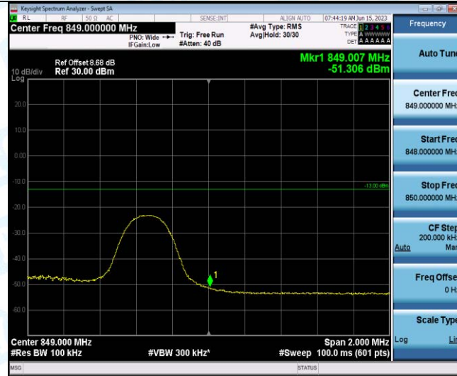
Band26-5MHz-QPSK-27015-1RB#24
