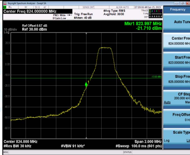
Band26-1.4MHz-QPSK-26797-1RB#5
