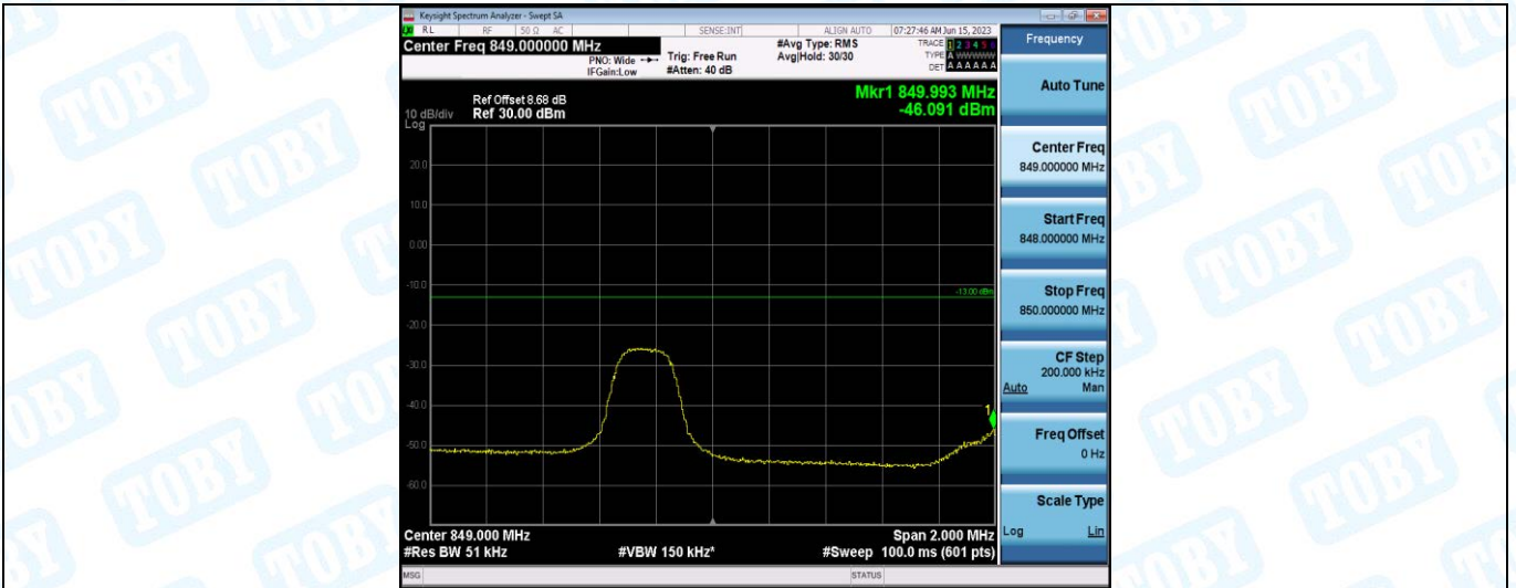
Band26-3MHz-16QAM-27025-1RB#14
