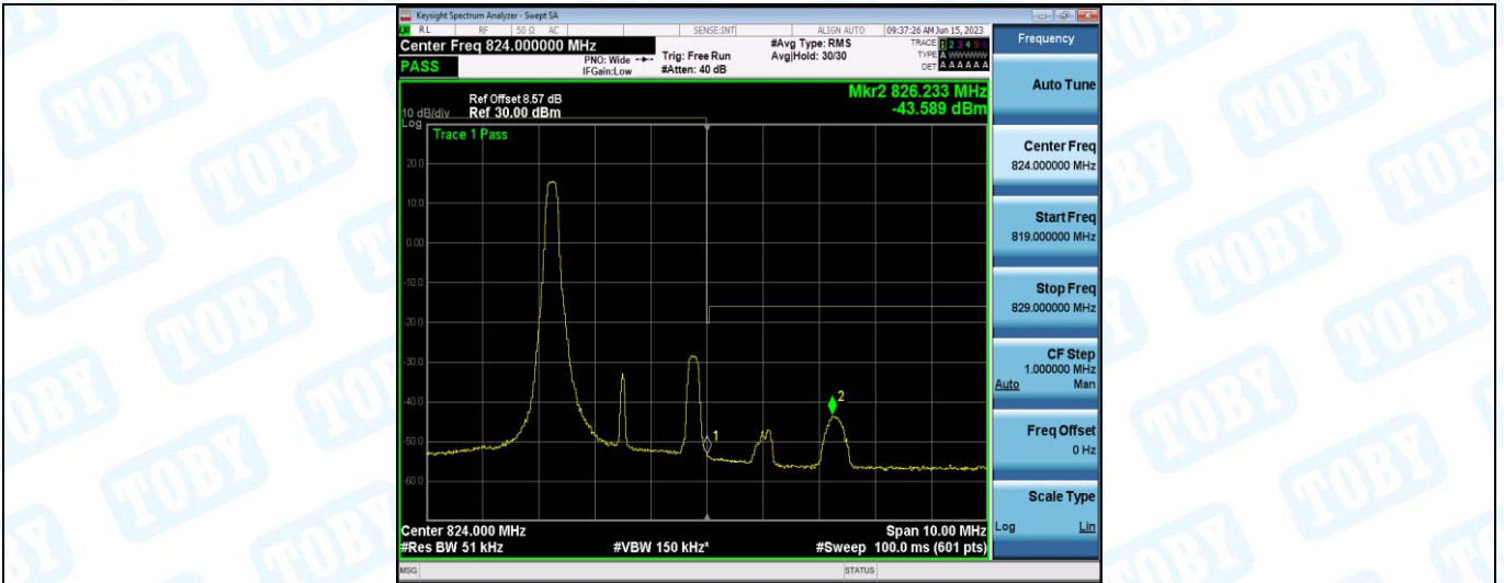
Band26-3MHz-16QAM-26775-1RB#14
