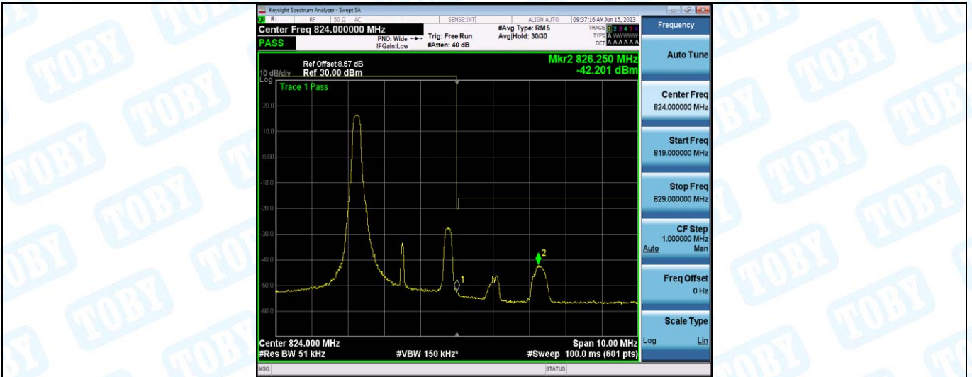
Band26-3MHz-QPSK-26775-1RB#14
