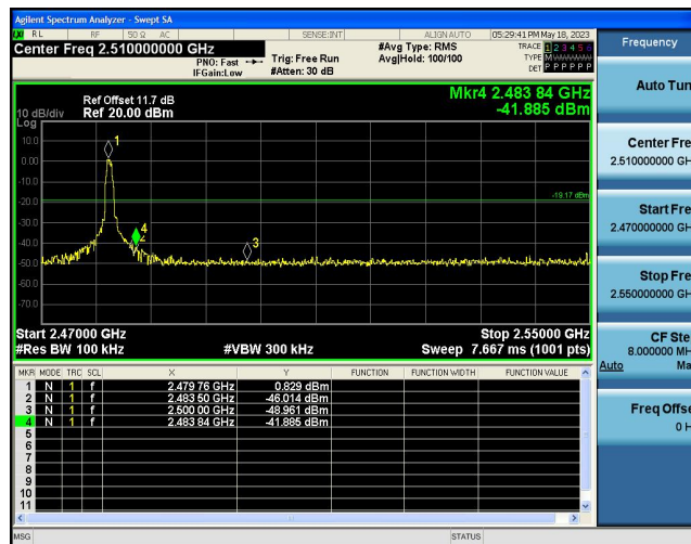
BLE_1M-Ant1-High-2480-0.83
