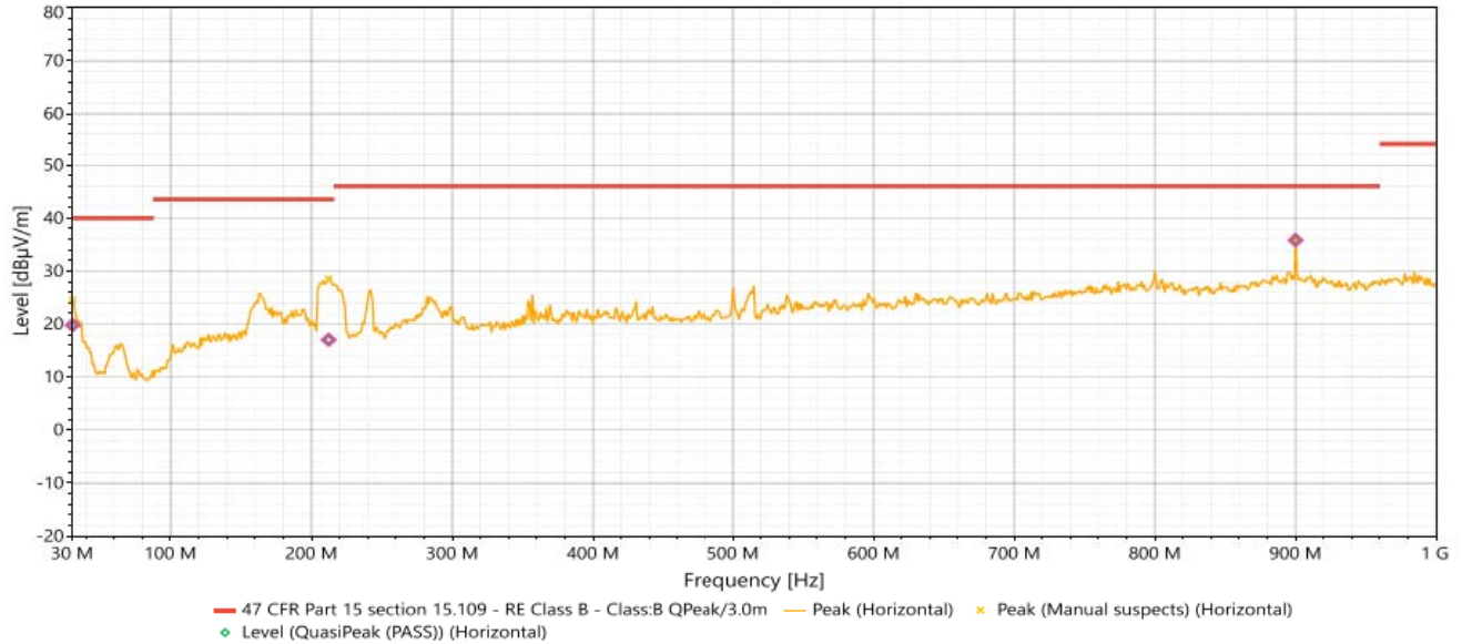
#2 - 30MHz-1GHz (Horizontal)
