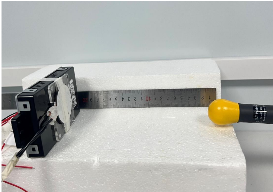
E-Field Test Setup Photo of Position E (20cm)
