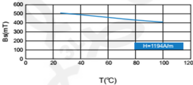
Bs—T Curve
