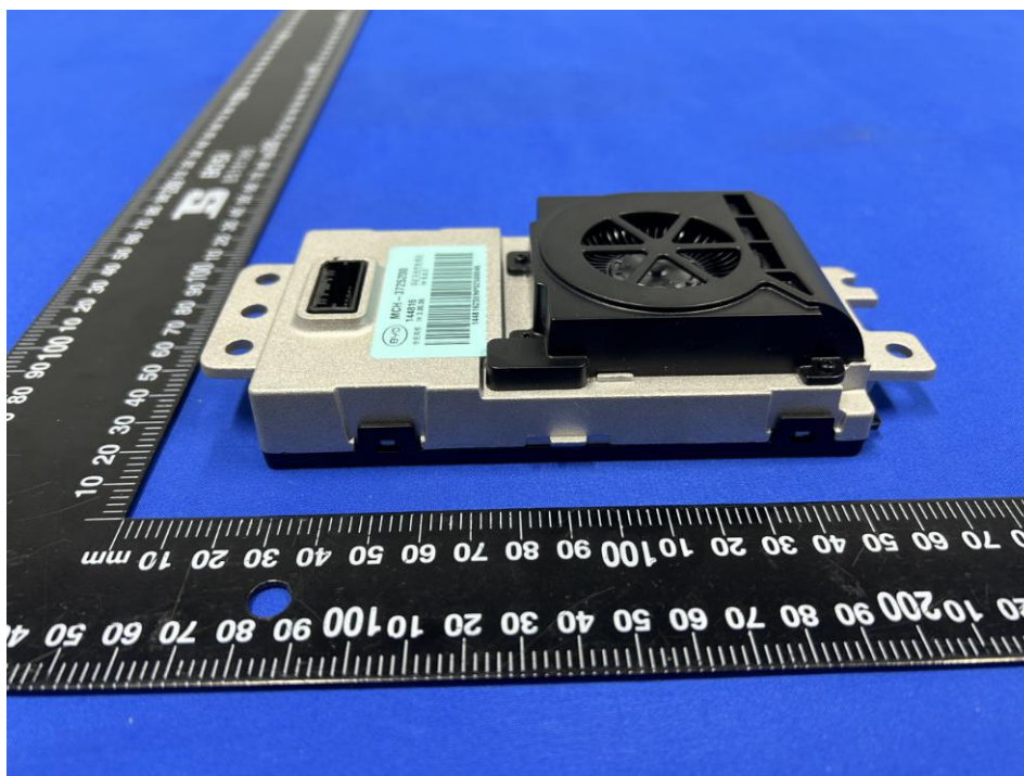
OUTSIDE VIEW OF EUT_MCH-3725200
