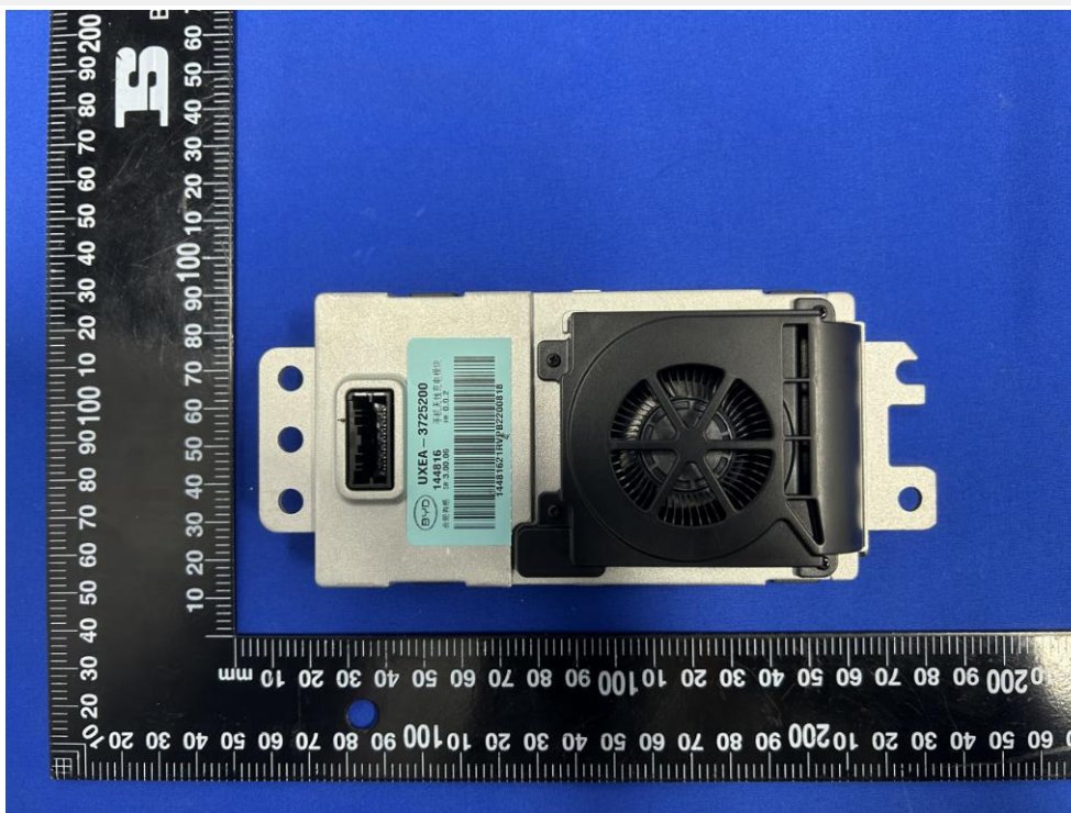
BACK SIDE VIEW OF EUT_UXEA-3725200
