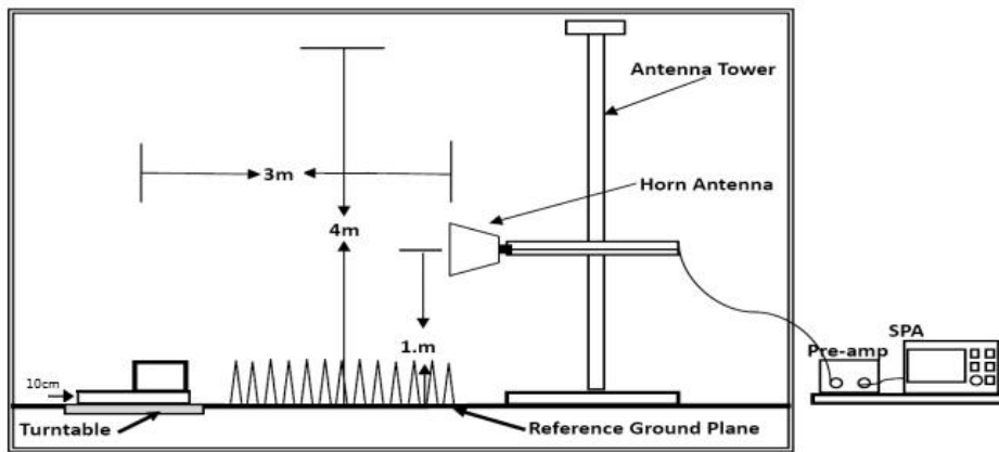
Above 1GHz
