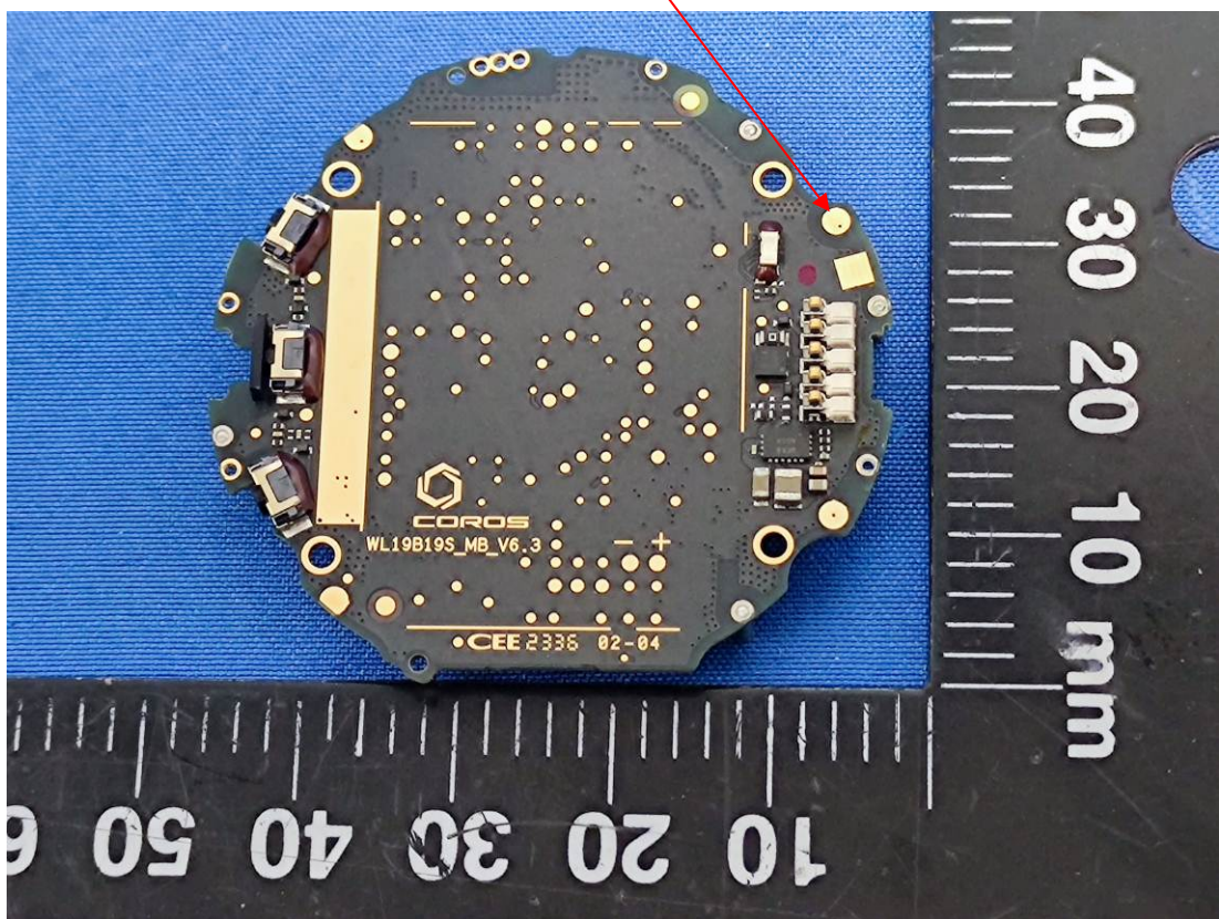
Antenna port
