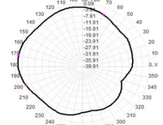
Total(H+V), Max: -1.62dB, CRD:13.29
