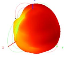
2480.0MHz H+V, ER: 42.4%
