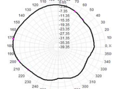
Total(H+V), Max: -1.32dB, CRD:11.26
