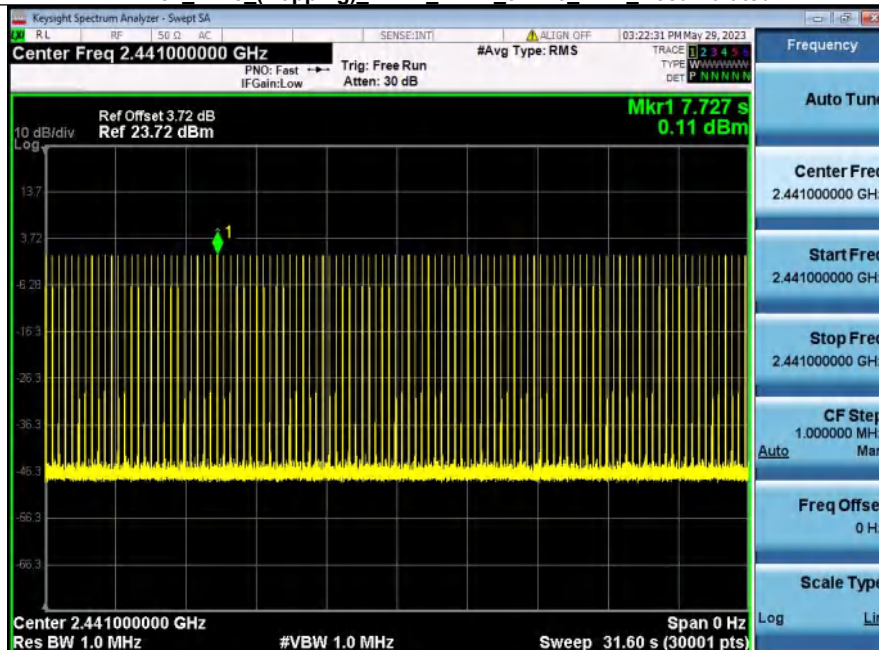
Dwell_Time_(Hopping)_NVNT_ANT1_3-DH5_2441_Accumulated
