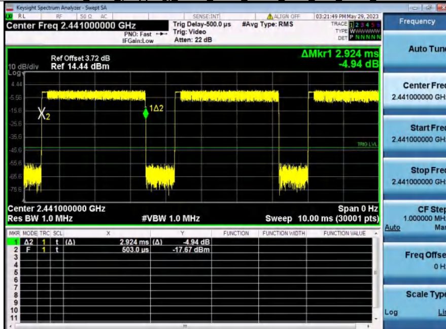
Dwell_Time_(Hopping)_NVNT_ANT1_3-DH5_2441_Accumulated
