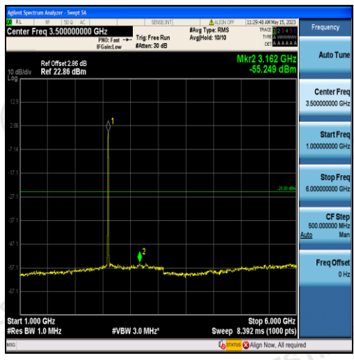
Band38-10MHz-16QAM-38000-50RB#0-Range2:1000~6000MHz
