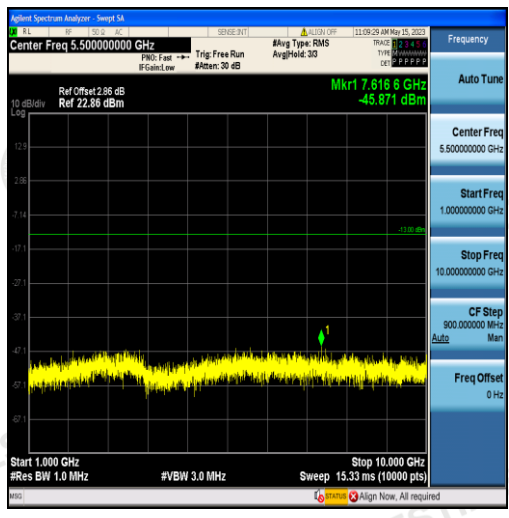
Band5-10MHz-16QAM-20525-50RB#0-Range2:1000~10000MHz
