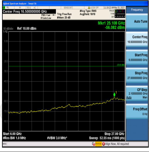
Band38-5MHz-16QAM-37775-25RB#0-Range3:6000~27000MHz
