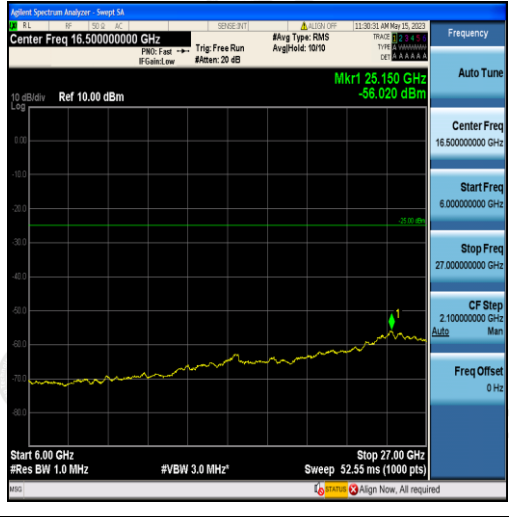
Band38-10MHz-16QAM-38200-50RB#0-Range3:6000~27000MHz
