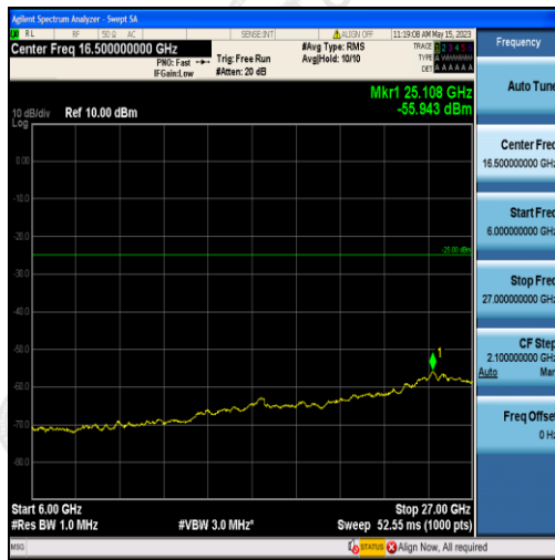
Band38-5MHz-QPSK-37775-25RB#0-Range3:6000~27000MHz
