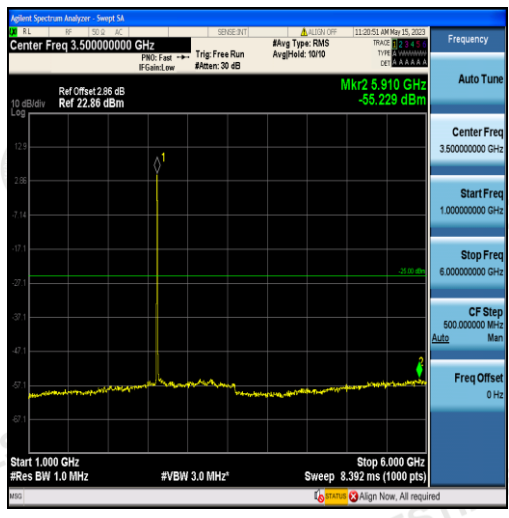
Band38-5MHz-16QAM-38225-25RB#0-Range2:1000~6000MHz
