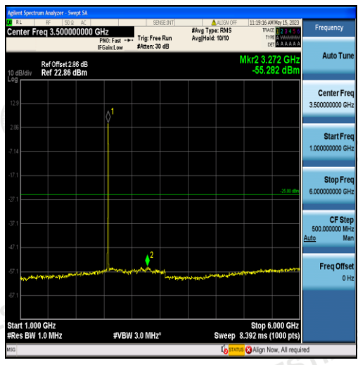
Band38-5MHz-16QAM-37775-25RB#0-Range2:1000~6000MHz
