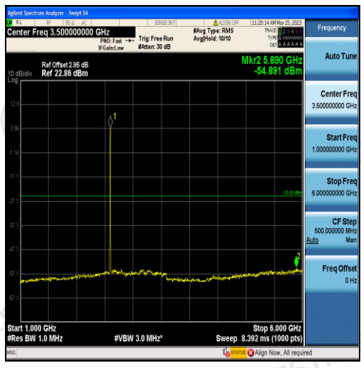
Band38-5MHz-16QAM-38000-25RB#0-Range2:1000~6000MHz
