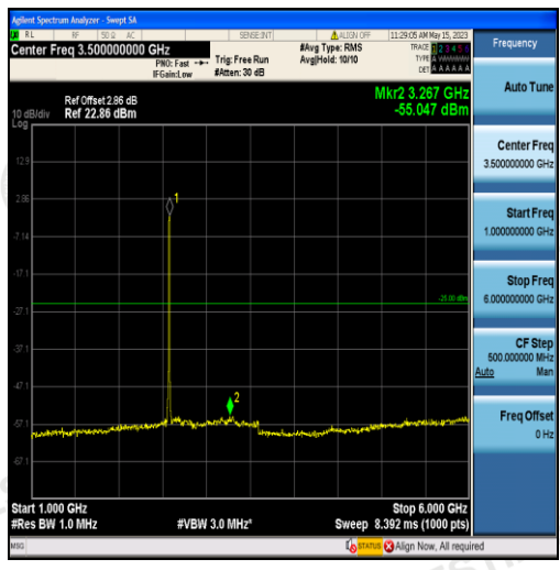
Band38-10MHz-16QAM-37800-50RB#0-Range2:1000~6000MHz
