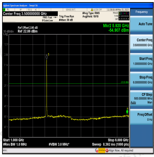
Band38-15MHz-16QAM-37825-75RB#0-Range2:1000~6000MHz
