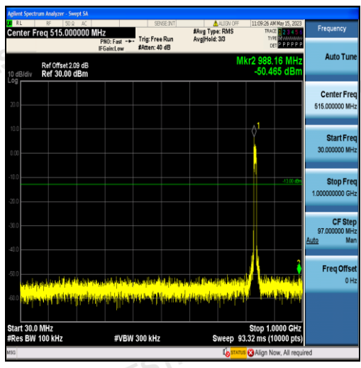
Band5-10MHz-16QAM-20525-50RB#0-Range1:30~1000MHz
