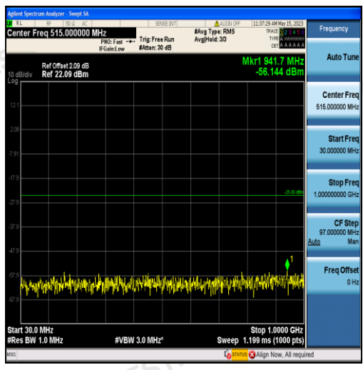
Band38-15MHz-QPSK-37825-75RB#0-Range1:30~1000MHz
