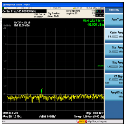
Band38-20MHz-QPSK-37850-100RB#0-Range1:30~1000MHz
