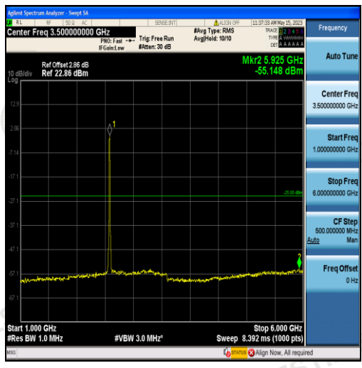
Band38-15MHz-QPSK-37825-75RB#0-Range2:1000~6000MHz
