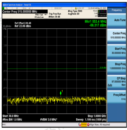
Band38-10MHz-16QAM-38000-50RB#0-Range1:30~1000MHz
