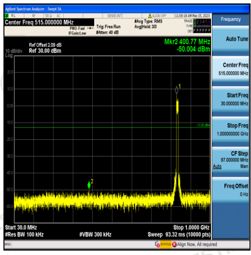
Band5-10MHz-QPSK-20525-50RB#0-Range1:30~1000MHz
