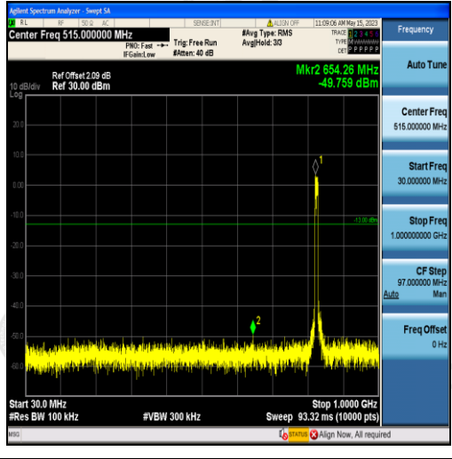
Band5-10MHz-16QAM-20450-50RB#0-Range1:30~1000MHz
