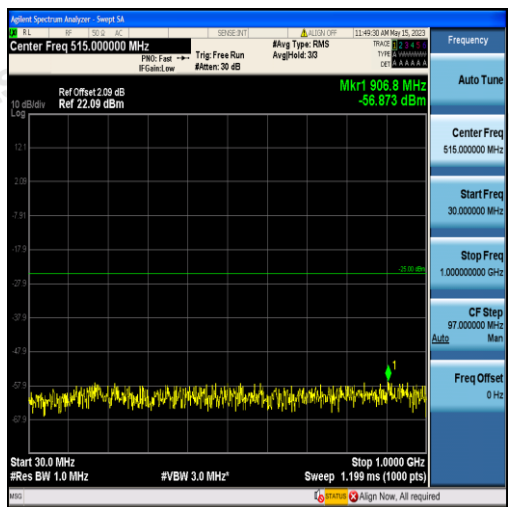
Band38-20MHz-QPSK-38000-100RB#0-Range1:30~1000MHz
