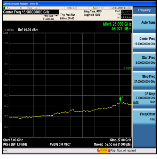
Band38-5MHz-16QAM-38225-25RB#0-Range3:6000~27000MHz
