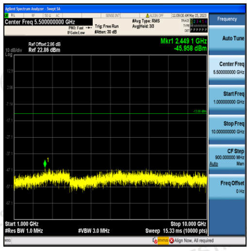
Band5-10MHz-QPSK-20450-50RB#0-Range2:1000~10000MHz
