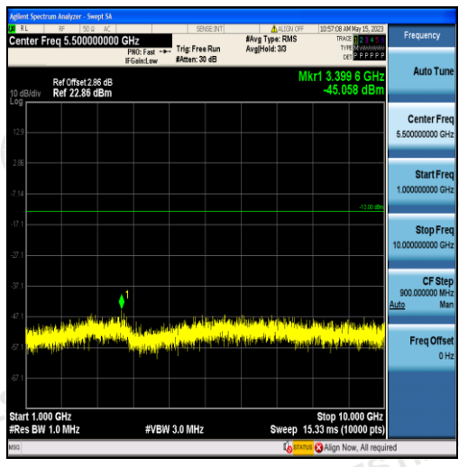
Band5-5MHz-16QAM-20525-25RB#0-Range2:1000~10000MHz
