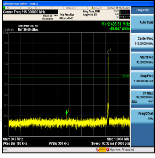
Band5-3MHz-16QAM-20415-15RB#0-Range1:30~1000MHz
