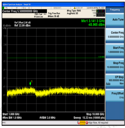
Band5-3MHz-16QAM-20525-15RB#0-Range2:1000~10000MHz
