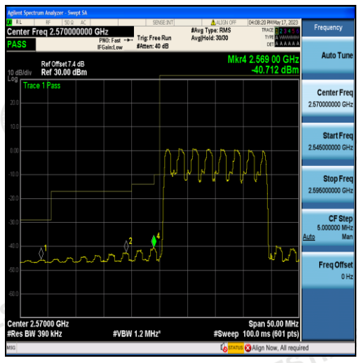
Band38-20MHz-16QAM-37850-100RB#0
