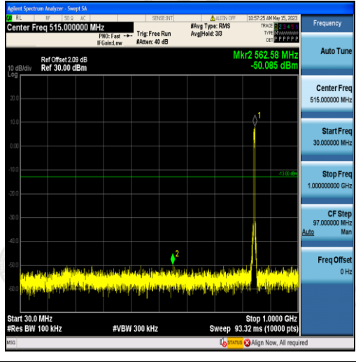
Band5-5MHz-QPSK-20625-25RB#0-Range1:30~1000MHz
