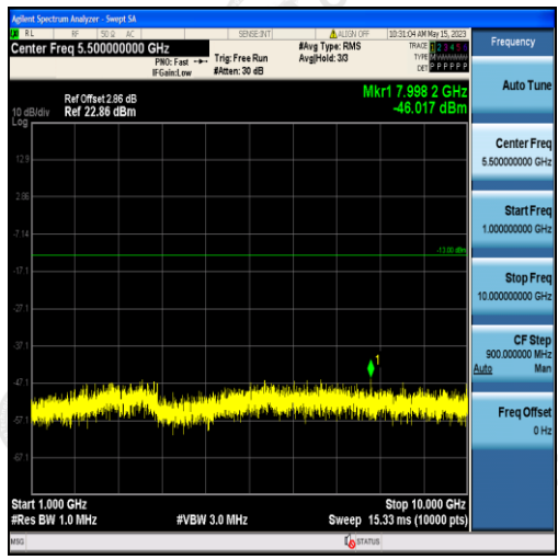
Band5-1.4MHz-16QAM-20643-6RB#0-Range2:1000~10000MHz
