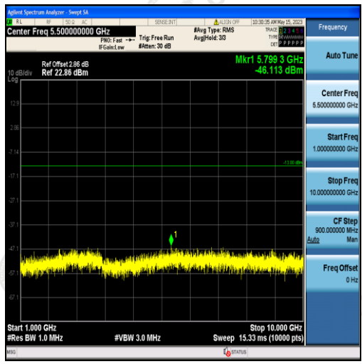
Band5-1.4MHz-QPSK-20525-6RB#0-Range2:1000~10000MHz
