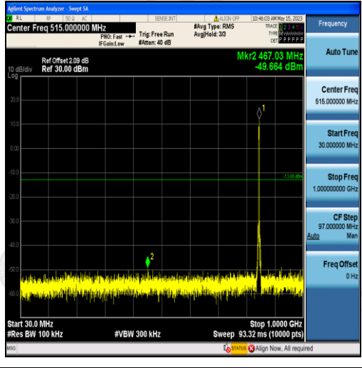
Band5-3MHz-QPSK-20635-15RB#0-Range1:30~1000MHz
