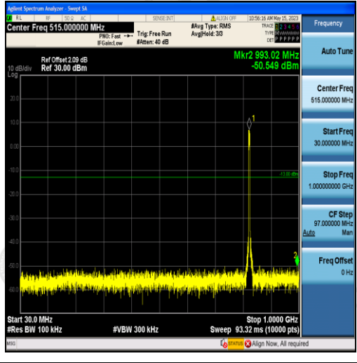
Band5-5MHz-16QAM-20425-25RB#0-Range1:30~1000MHz
