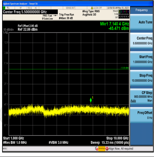
Band5-5MHz-QPSK-20525-25RB#0-Range2:1000~10000MHz
