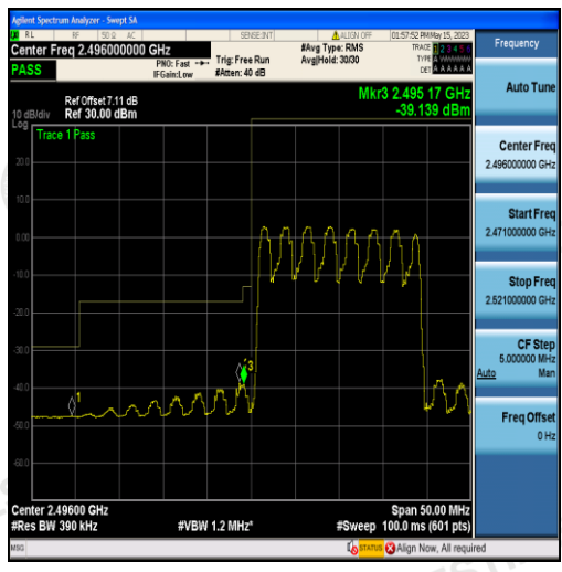
Band41-20MHz-QPSK-39750-100RB#0
