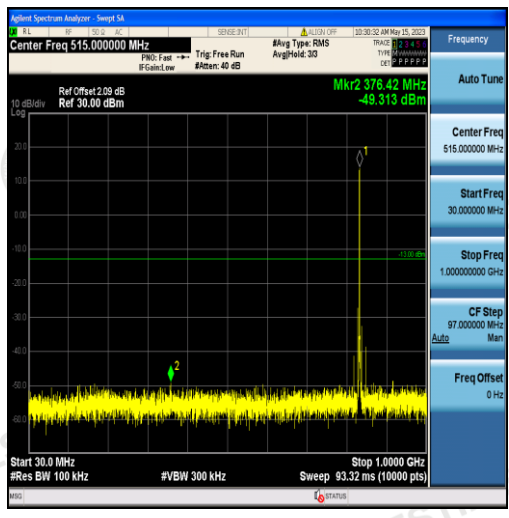
Band5-1.4MHz-QPSK-20525-6RB#0-Range1:30~1000MHz
