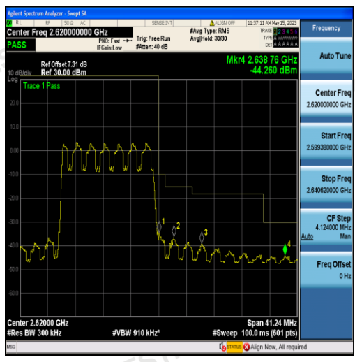
Band38-15MHz-QPSK-38175-75RB#0
