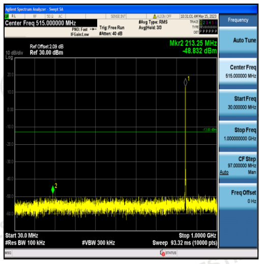
Band5-1.4MHz-16QAM-20643-6RB#0-Range1:30~1000MHz
