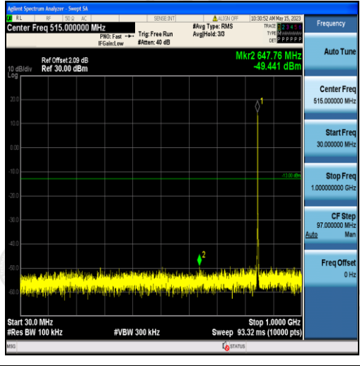
Band5-1.4MHz-QPSK-20643-6RB#0-Range1:30~1000MHz
