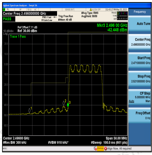
Band41-15MHz-16QAM-39725-75RB#0
