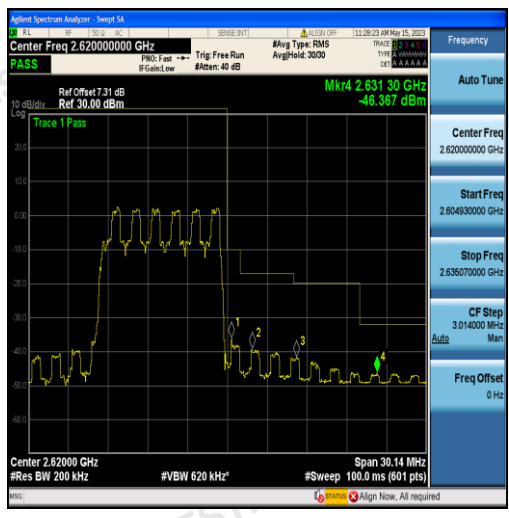
Band38-10MHz-QPSK-38200-50RB#0
