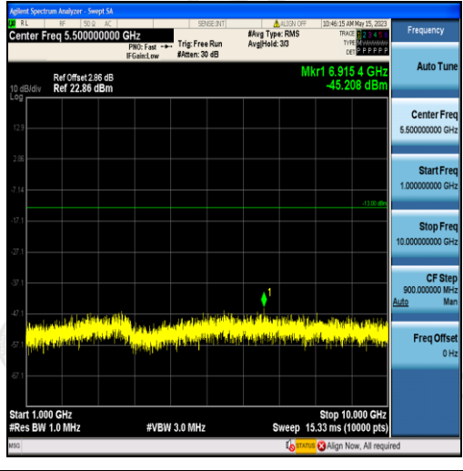
Band5-3MHz-16QAM-20635-15RB#0-Range2:1000~10000MHz
