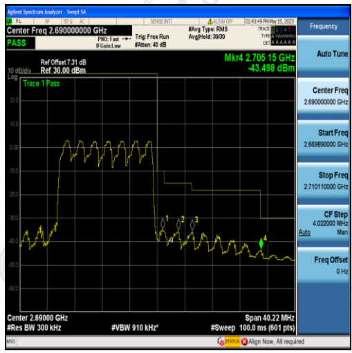
Band41-15MHz-QPSK-41515-75RB#0
