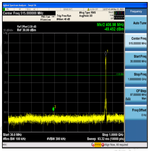
Band5-5MHz-16QAM-20625-25RB#0-Range1:30~1000MHz
