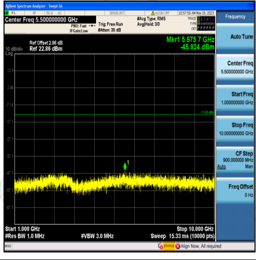
Band5-5MHz-16QAM-20625-25RB#0-Range2:1000~10000MHz
