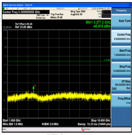
Band5-1.4MHz-16QAM-20407-6RB#0-Range2:1000~10000MHz
