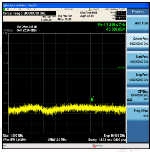
Band5-1.4MHz-QPSK-20407-6RB#0-Range2:1000~10000MHz
