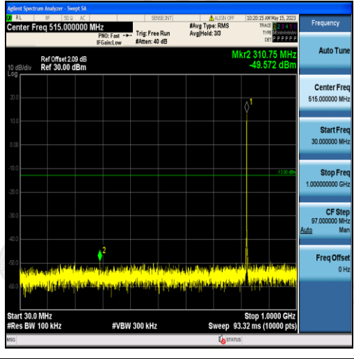
Band5-1.4MHz-16QAM-20407-6RB#0-Range1:30~1000MHz
