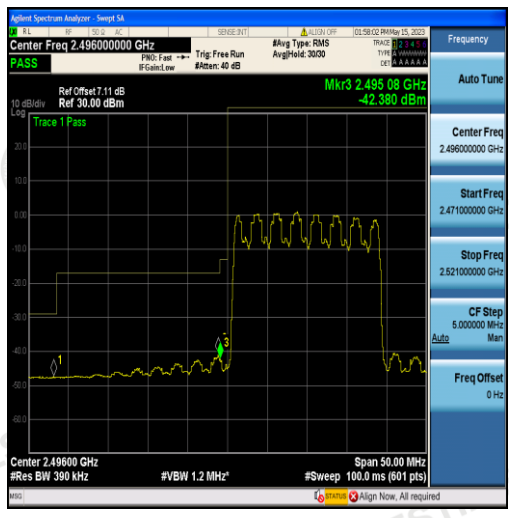
Band41-20MHz-16QAM-39750-100RB#0
