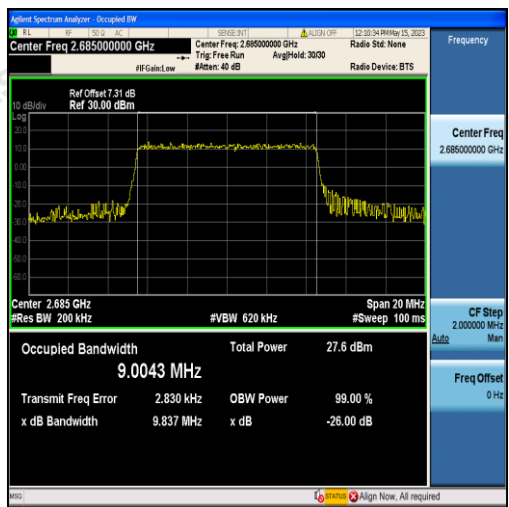
Band41-10MHz-16QAM-41540-50RB#0-9.0043
