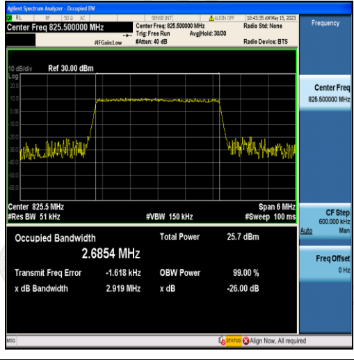
Band5-3MHz-16QAM-20415-15RB#0-2.6854
