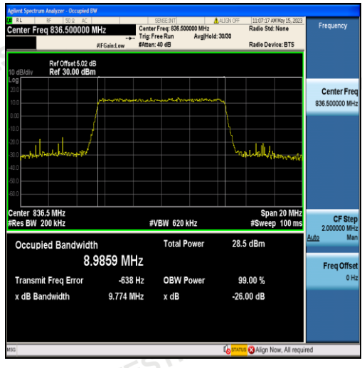
Band5-10MHz-QPSK-20525-50RB#0-8.9859
