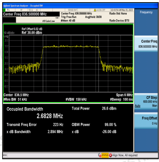
Band5-3MHz-16QAM-20525-15RB#0-2.6828
