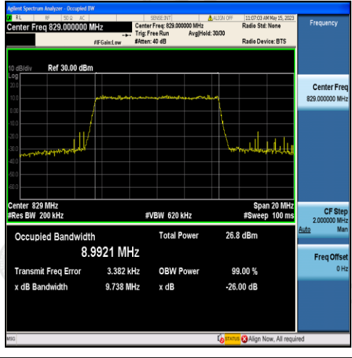
Band5-10MHz-16QAM-20450-50RB#0-8.9921
