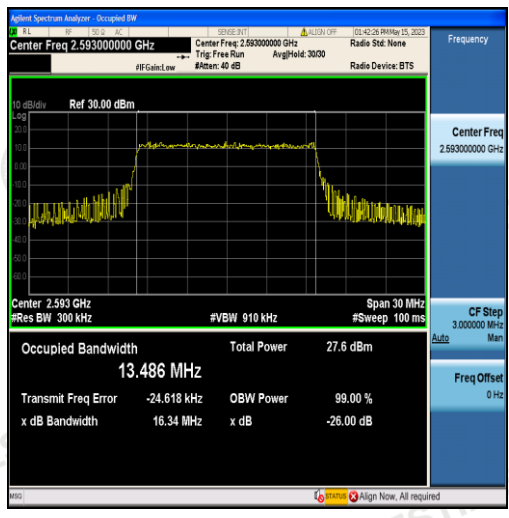
Band41-15MHz-16QAM-40620-75RB#0-13.486
