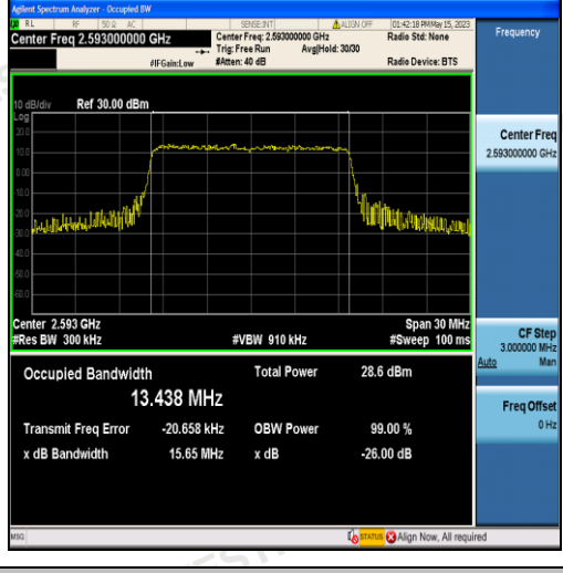
Band41-15MHz-QPSK-40620-75RB#0-13.438
