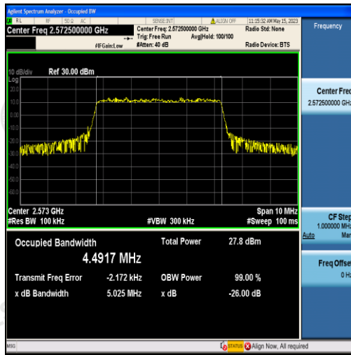
Band38-5MHz-QPSK-37775-25RB#0-4.4917
