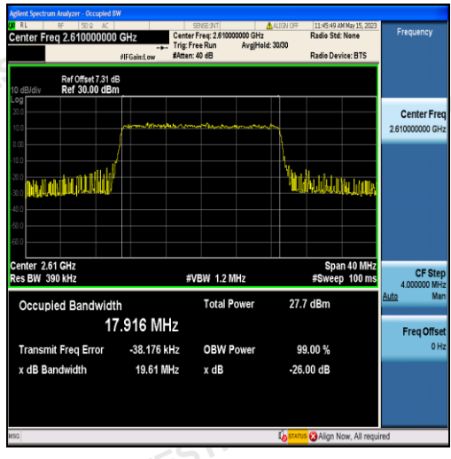
Band38-20MHz-16QAM-38150-100RB#0-17.916
