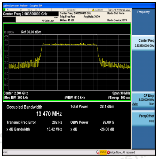
Band41-15MHz-QPSK-39725-75RB#0-13.470
