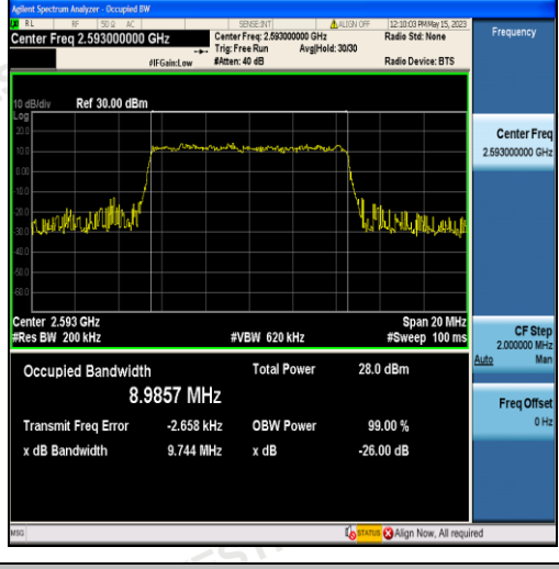
Band41-10MHz-QPSK-40620-50RB#0-8.9857
