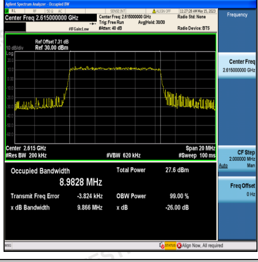
Band38-10MHz-16QAM-38200-50RB#0-8.9828
