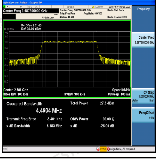
Band41-5MHz-16QAM-41565-25RB#0-4.4904
