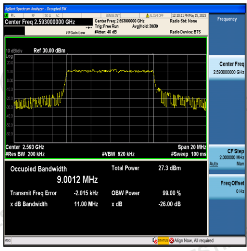
Band41-10MHz-16QAM-40620-50RB#0-9.0012
