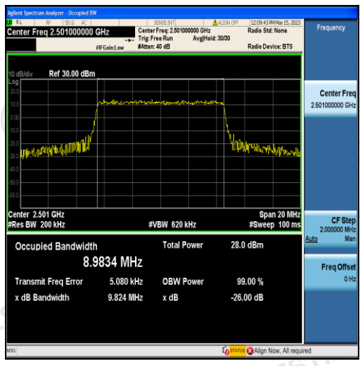
Band41-10MHz-QPSK-39700-50RB#0-8.9834
