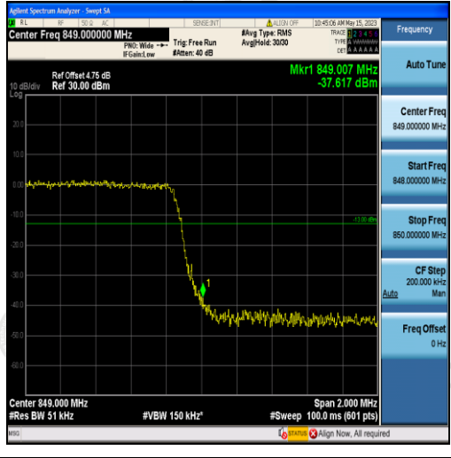
Band5-3MHz-16QAM-20635-15RB#0
