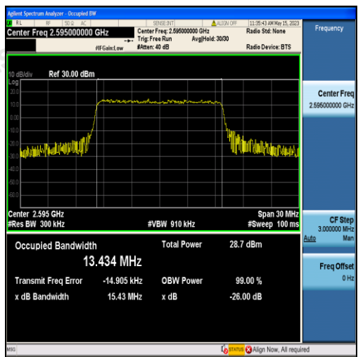
Band38-15MHz-QPSK-38000-75RB#0-13.434
