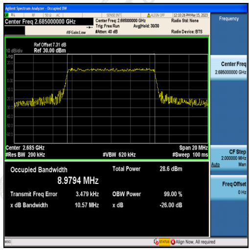
Band41-10MHz-QPSK-41540-50RB#0-8.9794
