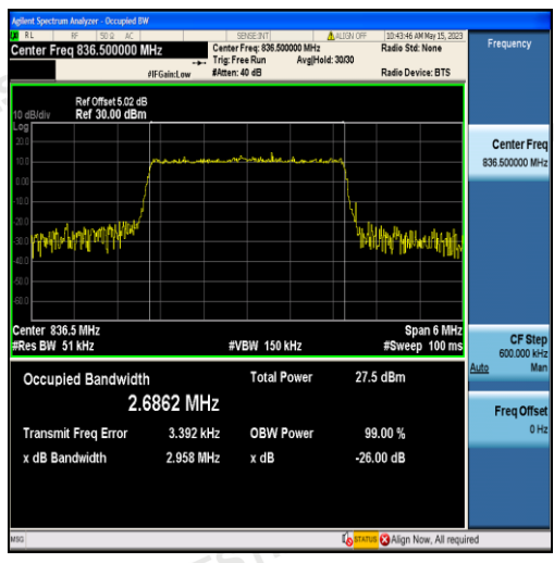
Band5-3MHz-QPSK-20525-15RB#0-2.6862
