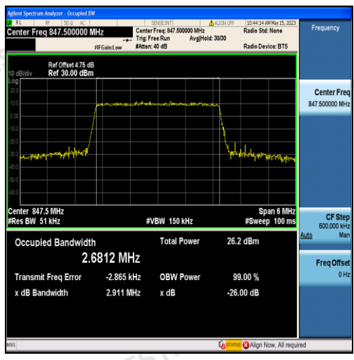
Band5-3MHz-16QAM-20635-15RB#0-2.6812
