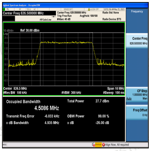
Band5-5MHz-QPSK-20425-25RB#0-4.5086
