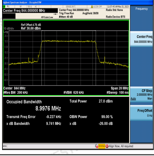
Band5-10MHz-16QAM-20600-50RB#0-8.9976
