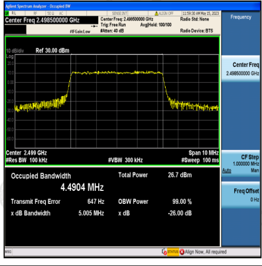
Band41-5MHz-16QAM-39675-25RB#0-4.4904
