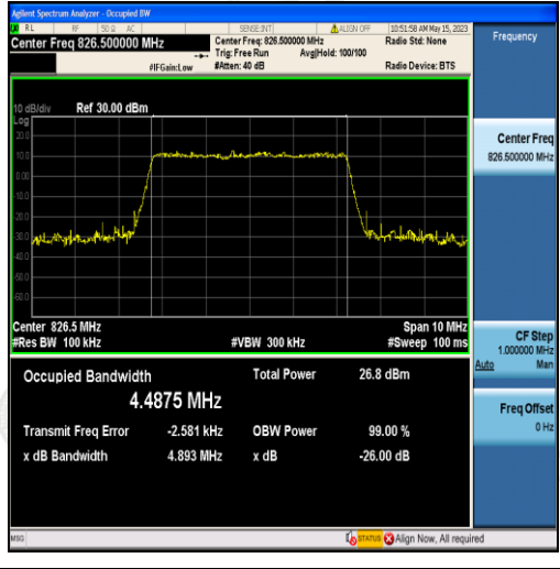
Band5-5MHz-16QAM-20425-25RB#0-4.4875
