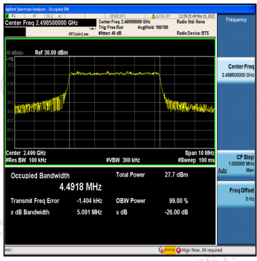
Band41-5MHz-QPSK-39675-25RB#0-4.4918
