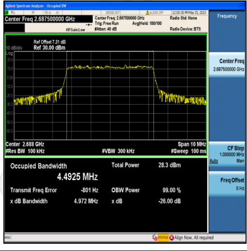
Band41-5MHz-QPSK-41565-25RB#0-4.4925
