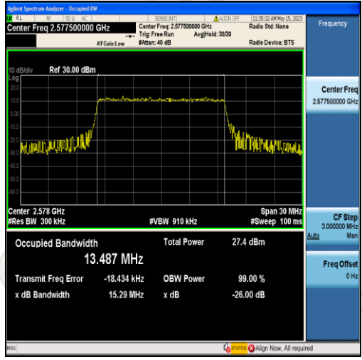
Band38-15MHz-16QAM-37825-75RB#0-13.487
