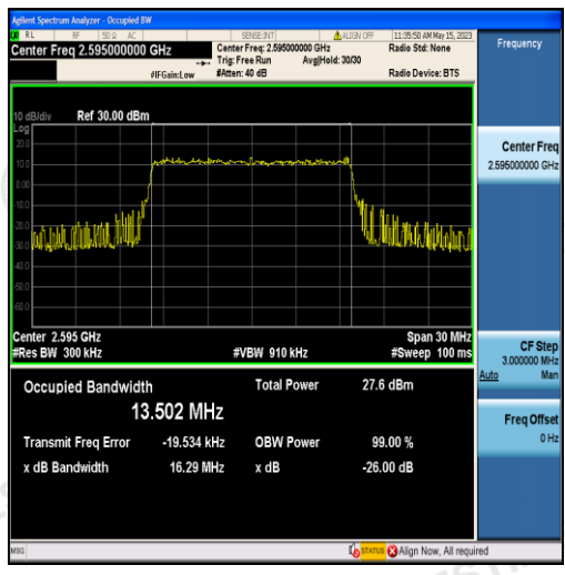
Band38-15MHz-16QAM-38000-75RB#0-13.502
