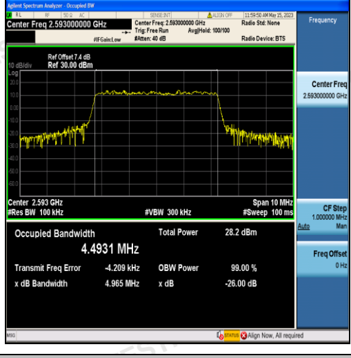
Band41-5MHz-QPSK-40620-25RB#0-4.4931
