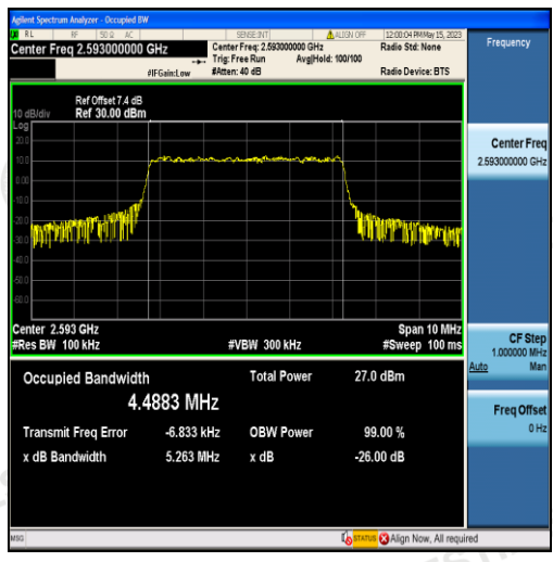
Band41-5MHz-16QAM-40620-25RB#0-4.4883
