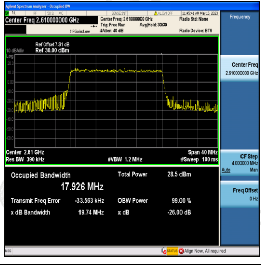
Band38-20MHz-QPSK-38150-100RB#0-17.926
