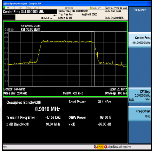
Band5-10MHz-QPSK-20600-50RB#0-8.9818
