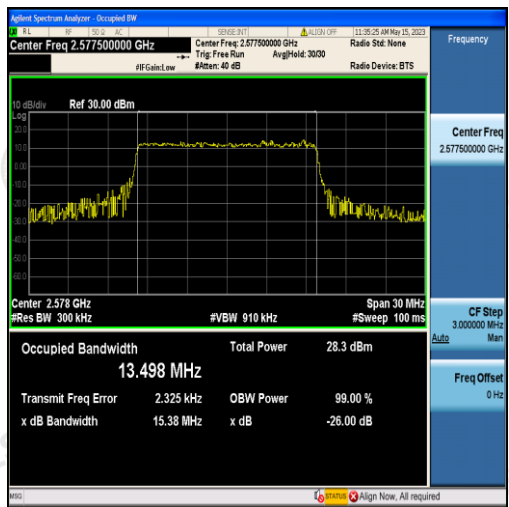
Band38-15MHz-QPSK-37825-75RB#0-13.498
