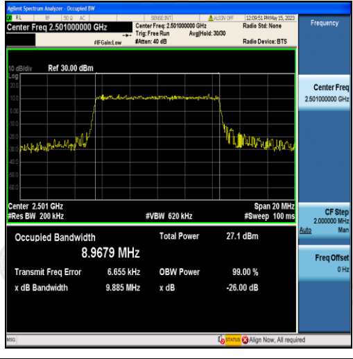
Band41-10MHz-16QAM-39700-50RB#0-8.9679
