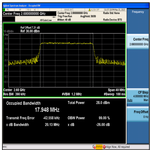
Band41-20MHz-16QAM-41490-100RB#0-17.948
