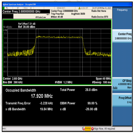
Band41-20MHz-QPSK-41490-100RB#0-17.920
