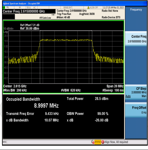
Band38-10MHz-QPSK-38200-50RB#0-8.9997
