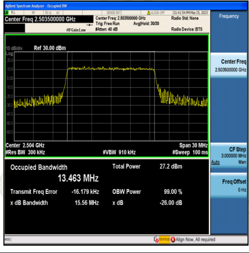
Band41-15MHz-16QAM-39725-75RB#0-13.463
