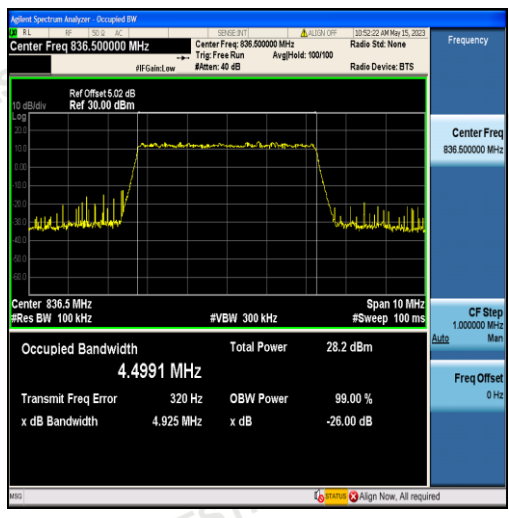
Band5-5MHz-QPSK-20525-25RB#0-4.4991
