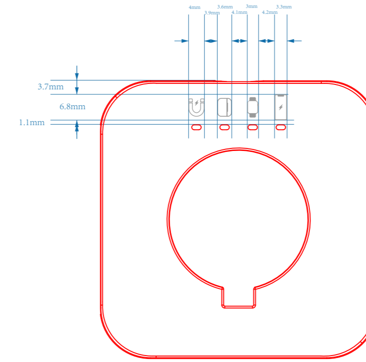
Watch cover
