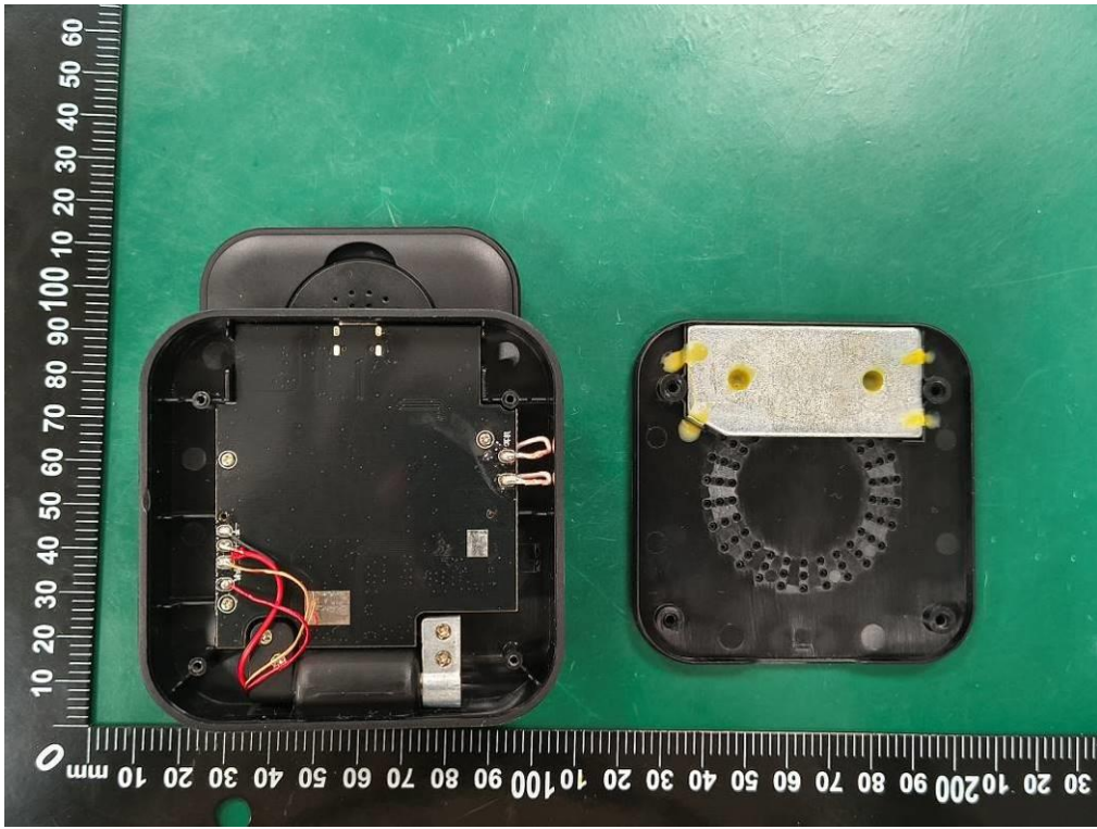
Internal Photo FCC ID: 2BBEH-W377
