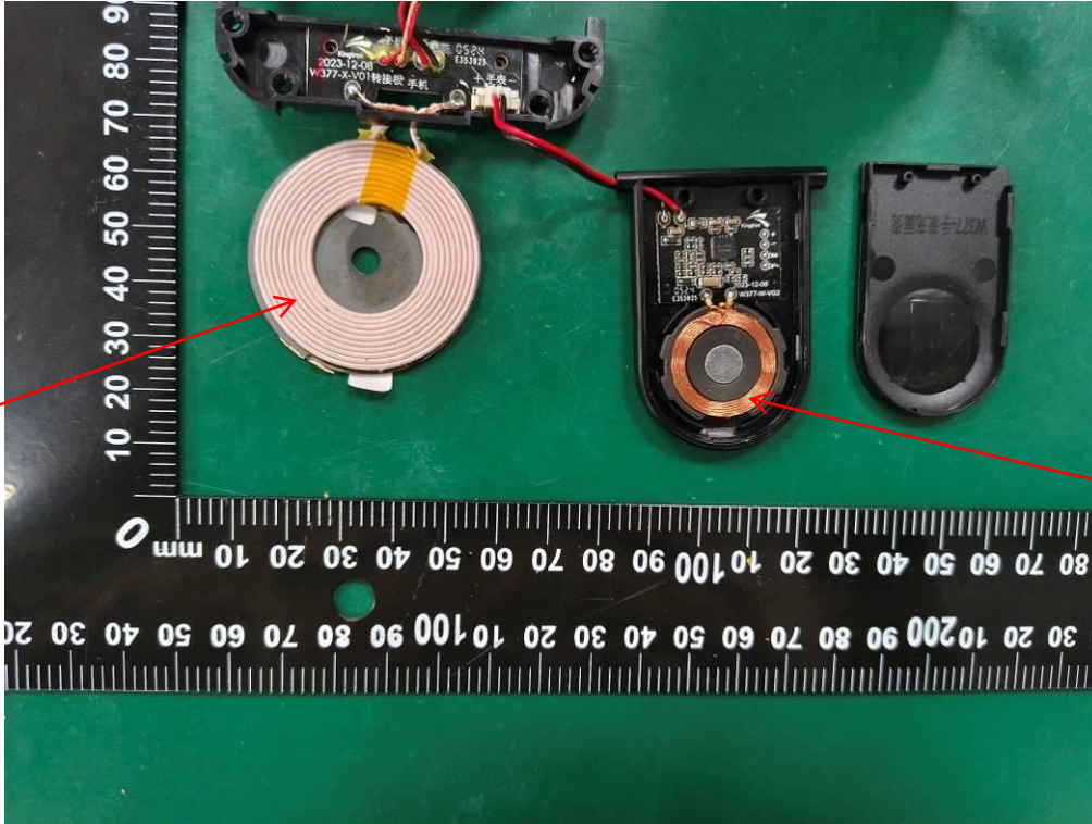
ANT for Phone
