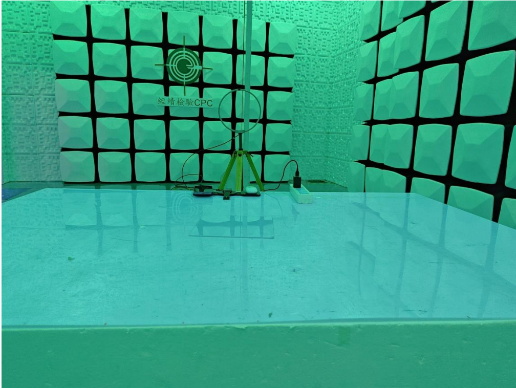
Setup Photo FCC ID: 2BBEH-W375
