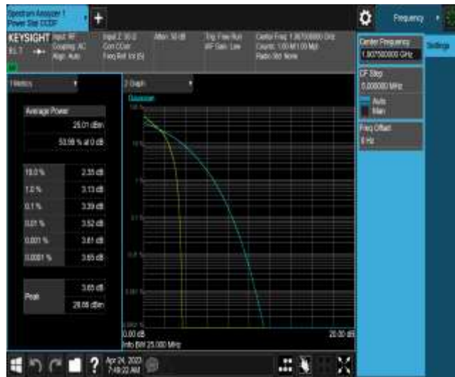
Band25-15MHz-QPSK-26615-1RB#0
