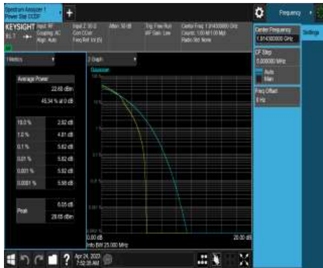
Band25-1.4MHz-16QAM-26683-1RB#0
