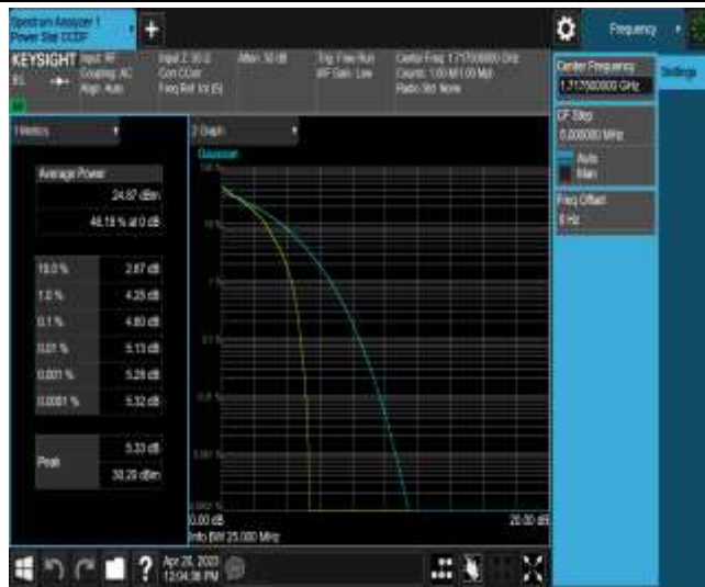
Band4-15MHz-QPSK-2025-1RB#0
