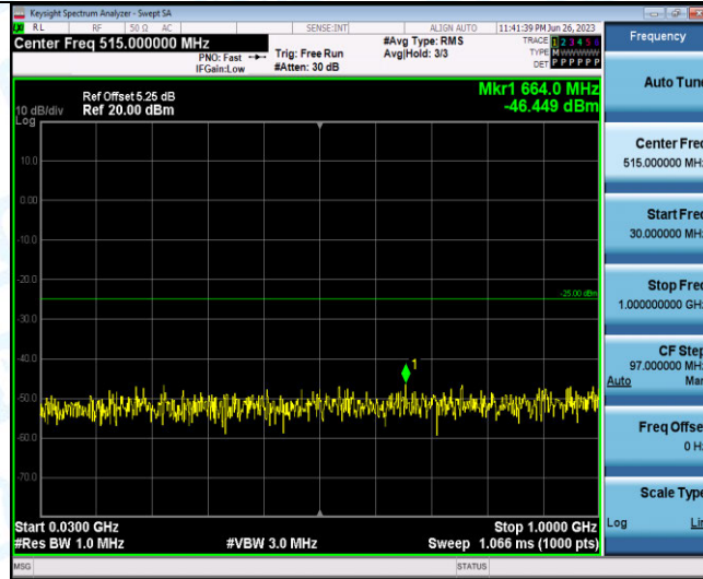
Band41-15MHz-16QAM-41165-1RB#0-Range3:30~1000MHz
