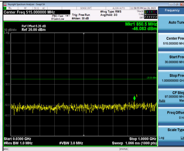
Band41-20MHz-QPSK-40640-1RB#0-Range3:30~1000MHz
