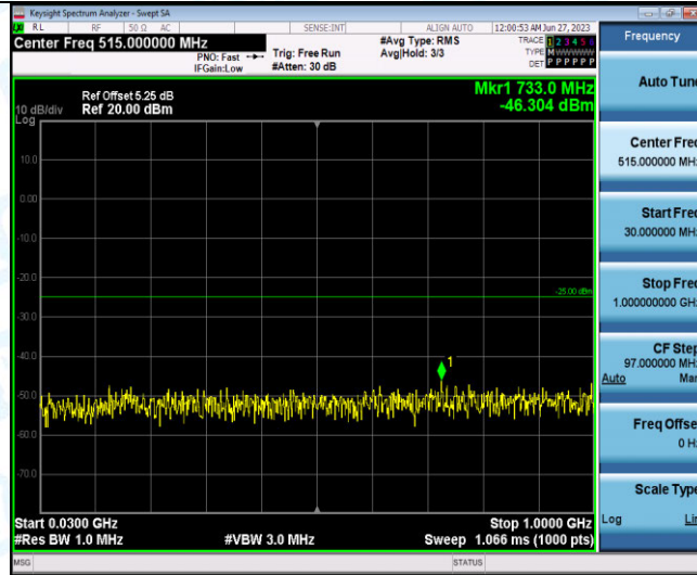
Band41-20MHz-16QAM-41140-1RB#0-Range3:30~1000MHz
