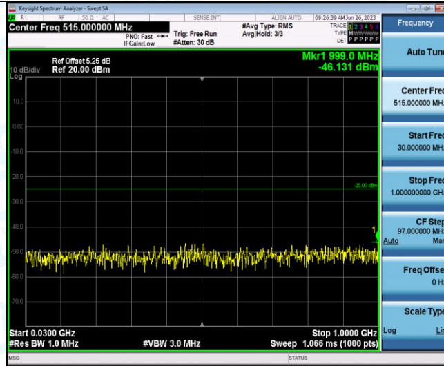
Band41-10MHz-QPSK-41190-1RB#0-Range1:30~1000MHz
