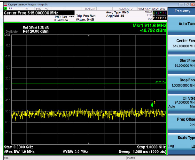
Band41-10MHz-QPSK-40640-1RB#0-Range3:30~1000MHz
