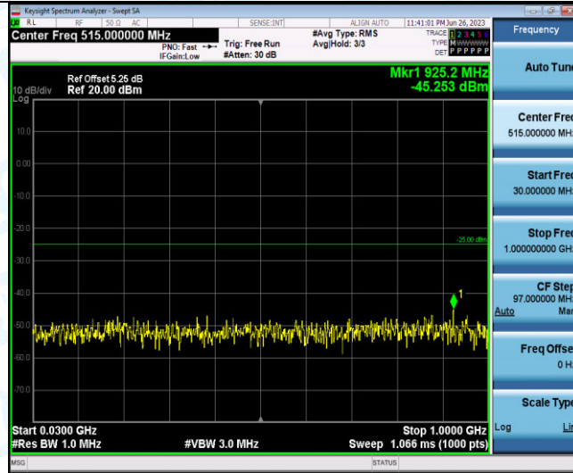
Band41-15MHz-QPSK-41165-1RB#0-Range3:30~1000MHz
