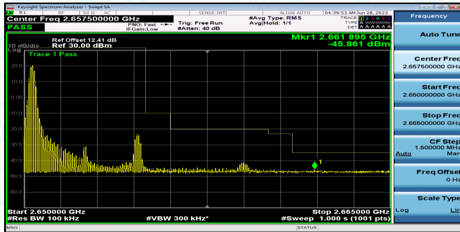
Band41_Band41_5MHz_QPSK_41215_1RB#0
