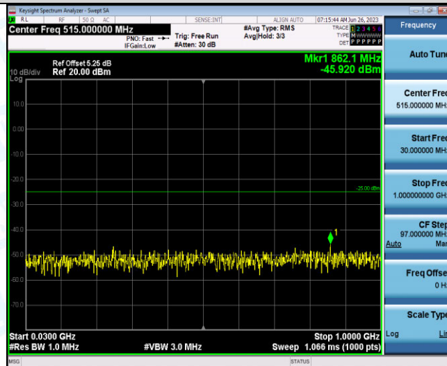
Band41-5MHz-QPSK-40640-1RB#0-Range3:30~1000MHz
