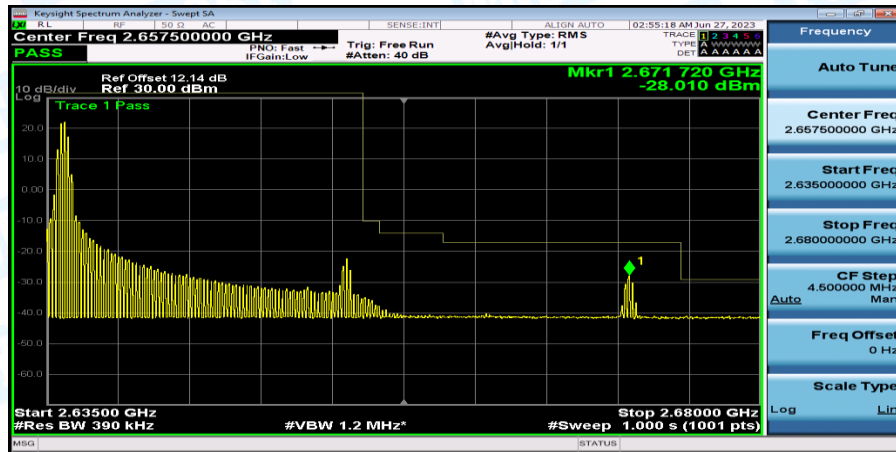
Band41_Band41_20MHz_16QAM_41140_1RB#0
