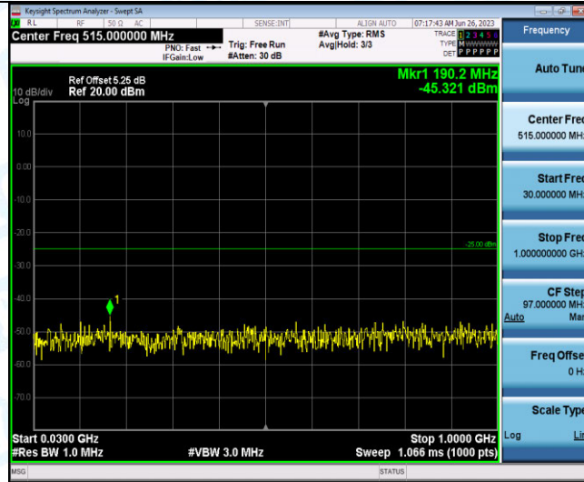
Band41-5MHz-QPSK-41215-1RB#0-Range3:30~1000MHz
