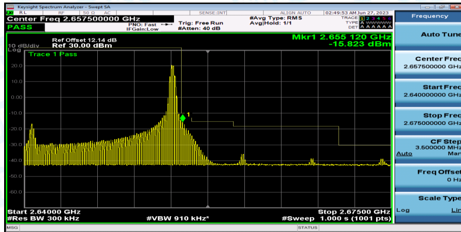
Band41_Band41_15MHz_16QAM_41165_1RB#74
