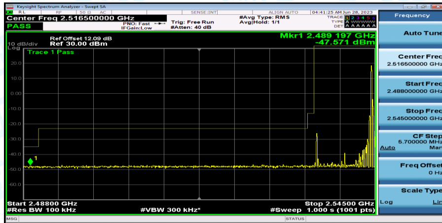
Band41_Band41_10MHz_16QAM_40090_1RB#49
