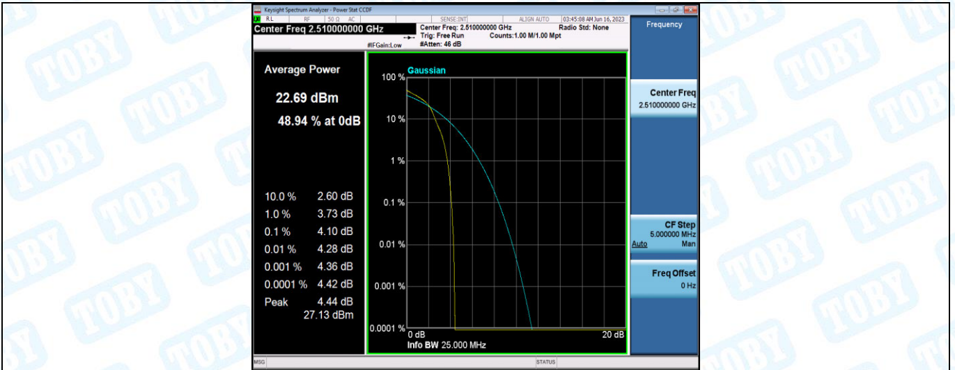
Band7-20MHz-16QAM-20850-27RB#0
