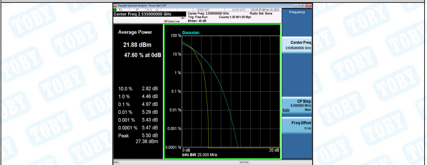
Band7-20MHz-16QAM-21100-27RB#0
