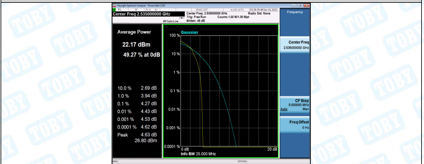
Band7-10MHz-16QAM-21100-27RB#0
