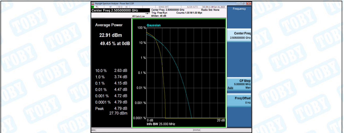
Band7-10MHz-16QAM-20800-27RB#0
