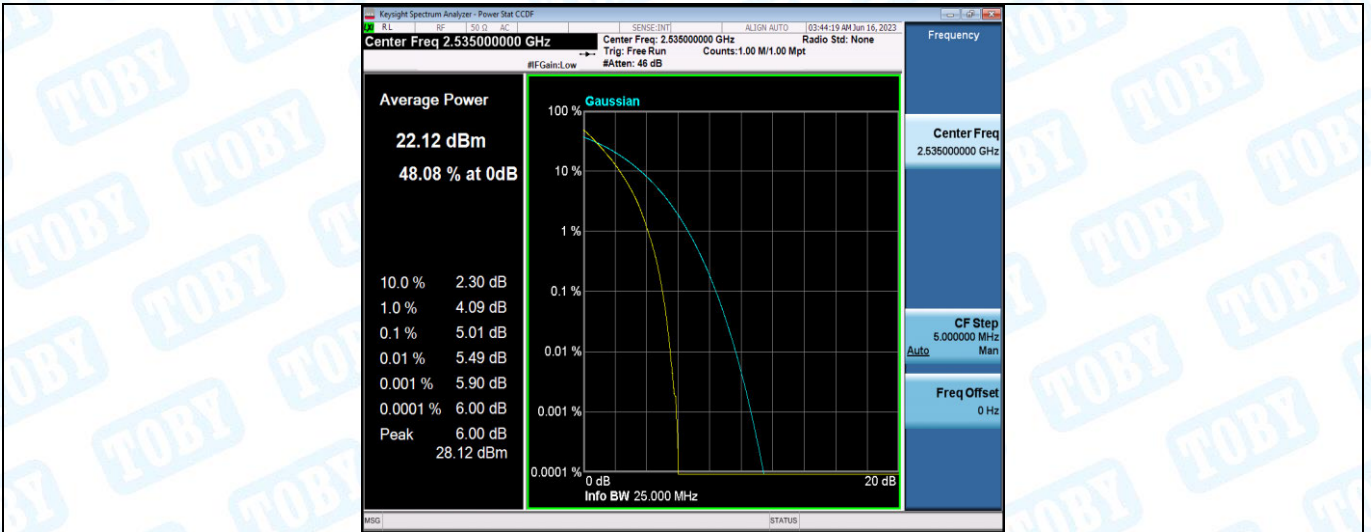
Band7-20MHz-QPSK-21350-1RB#0
