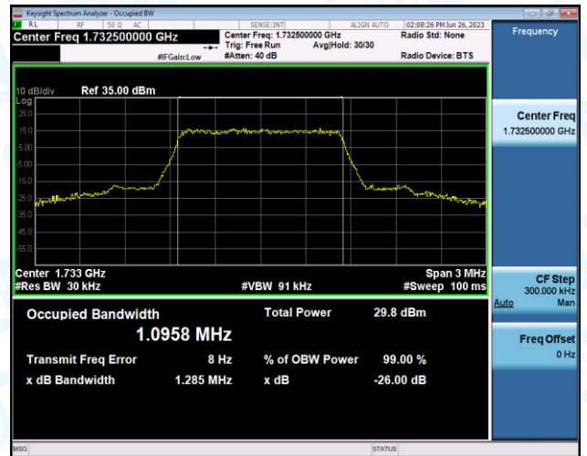
Band4-1.4MHz-16QAM-20393-6RB#0-PASS
