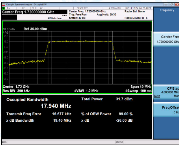
Band4-20MHz-QPSK-20300-100RB#0-PASS
