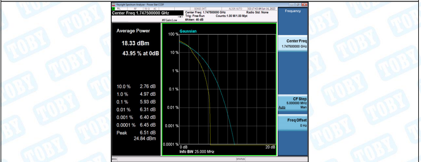
Band4-15MHz-16QAM-20325-27RB#0
