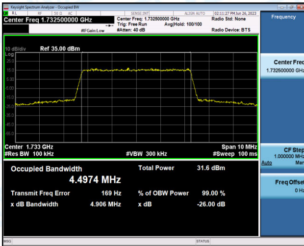
Band4-5MHz-QPSK-20375-25RB#0-PASS
