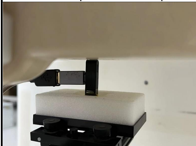
Vertical-Front of EUT with 0 cm Gap
