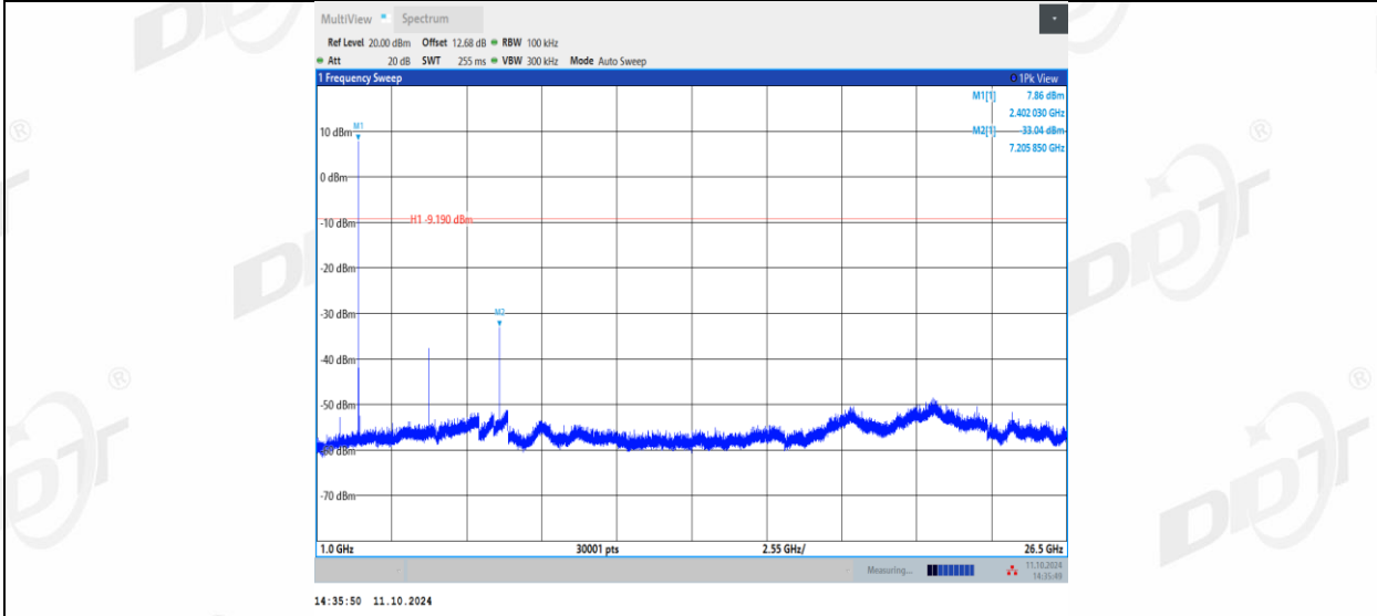
3DH5_Ant1_2441_0~Reference
