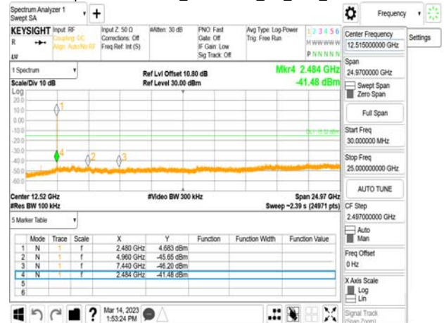
Spurious Emission_π/4QPSK_2M_DH5_2480MHz
