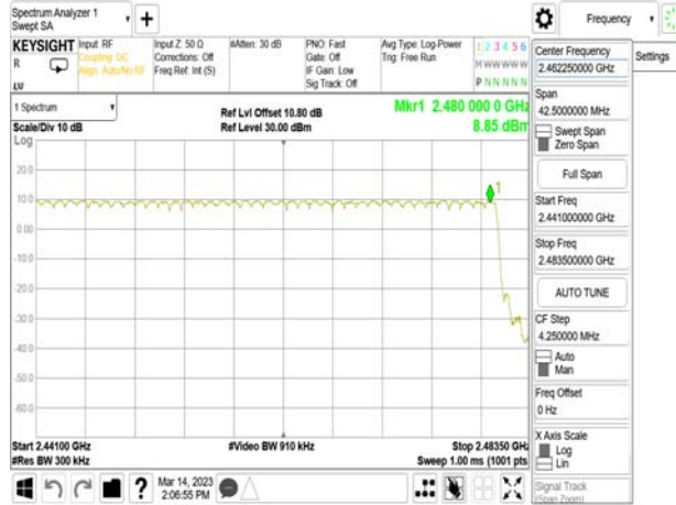
\pi/4 DQPSK_2M_DH5_2441-2480
