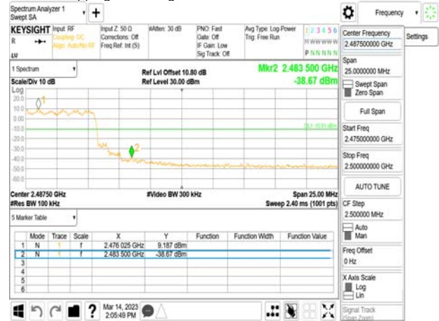
Hopping Band Edge_π/4DQPSK_2M_DH5_2480MHz
