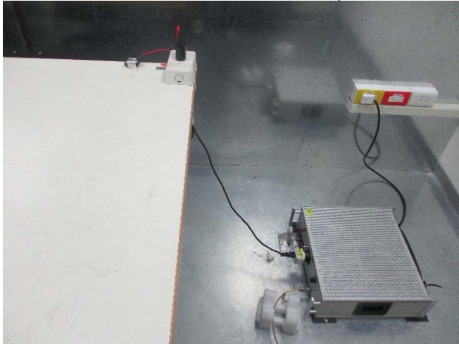
Part_15_247_LE_Conduction_Setup
