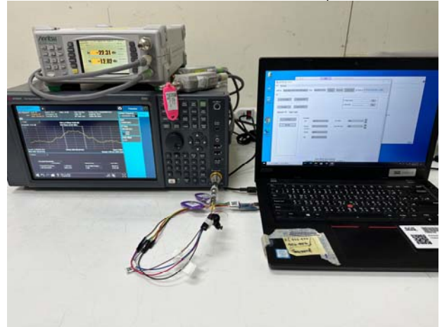
Part_15_247_LE_Conducted_Setup
