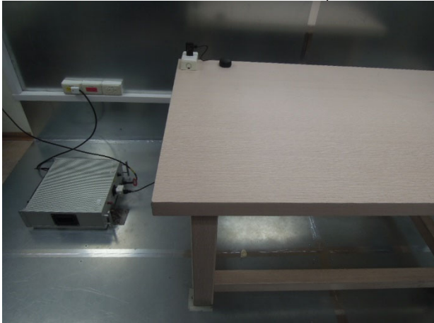
FCC_15_247_BT_Conduction_setup
