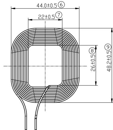
L1L3绕线尺寸(小R角),L1为L3的镜像,11 Truns
