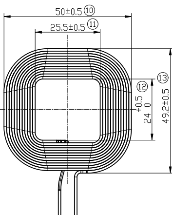
L2:绕线尺寸(小R角),12 Truns
