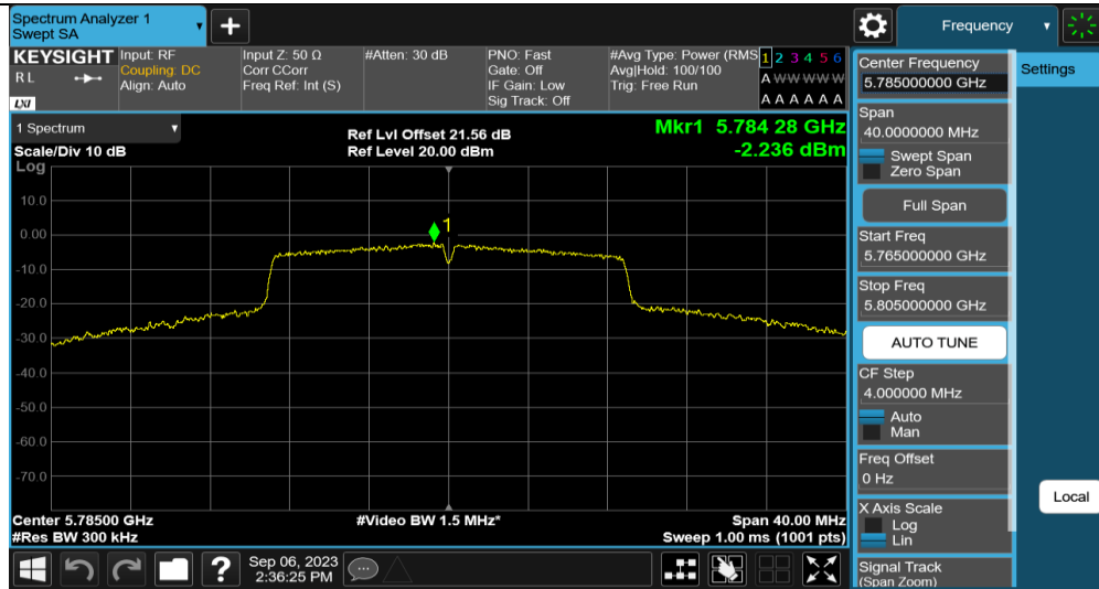
11N20MIMO Ant2 5785
