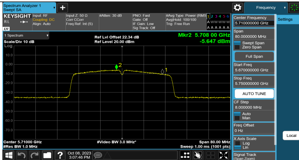
11N40MIMO Ant2 5710
