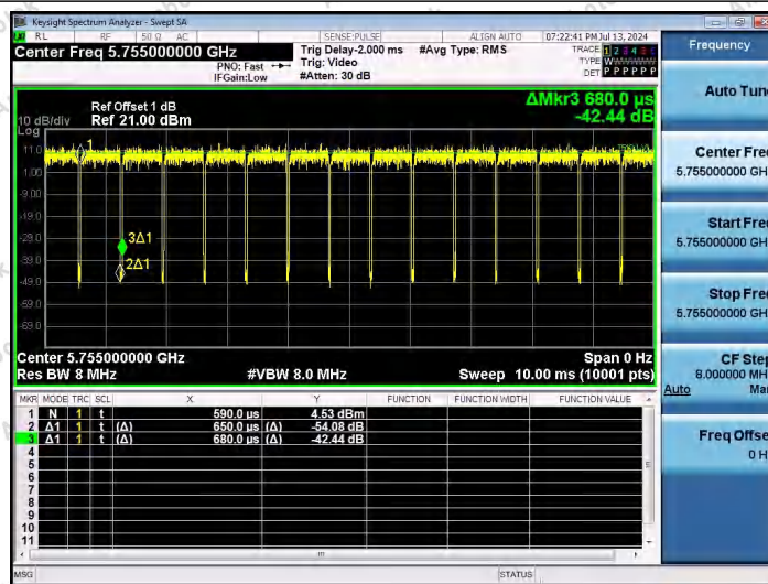
NTNV-11N40SISO-Ant1-5755
