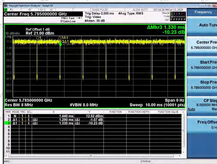
NTN-11N20SISO-Ant1-5785
