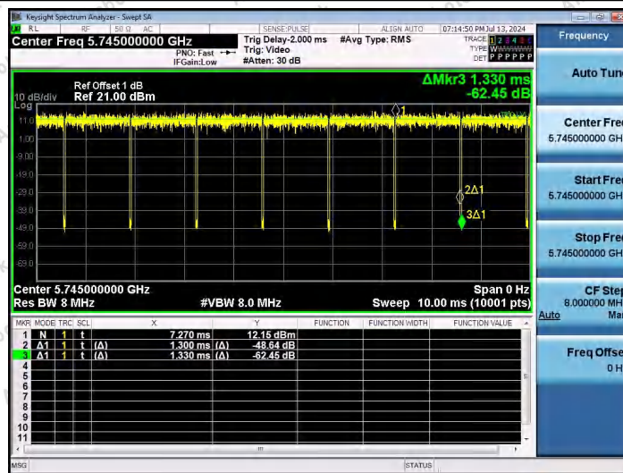
NTN-11N20SISO-Ant1-5745
