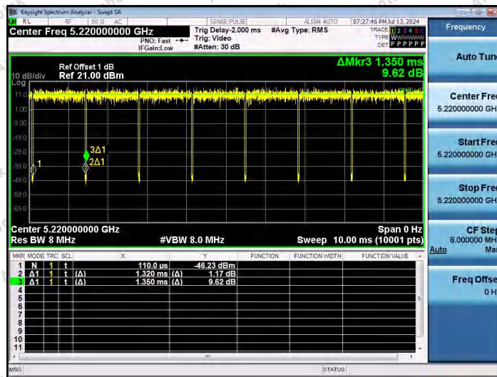
NTVN-11AC20SISO-Ant1-5220
