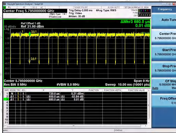
NTVN-11N40SISO-Ant1-5795
