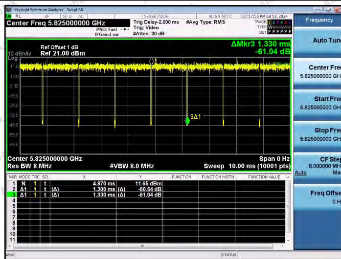
NTN-11N20SISO-Ant1-5825
