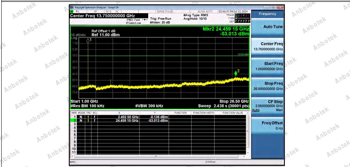
DH5-Ant1-2402-1000~26500-PASS
