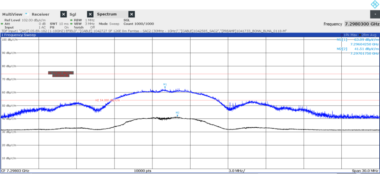
Fig. 20: Final Measurement – Unwanted emission in restricted band
