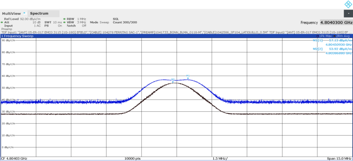
Fig. 39: Sample #2. Mode 1. Spurious Emission 4804 MHz. Channel Low
