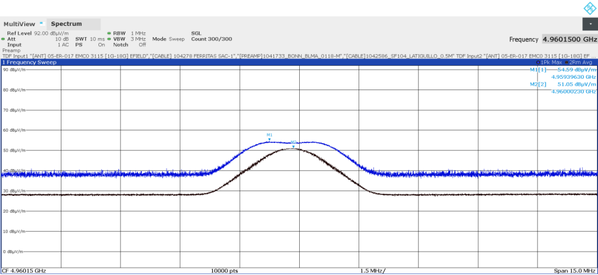
Fig. 43: Sample #2. Mode 1. Spurious Emission 4960 MHz. Channel High
