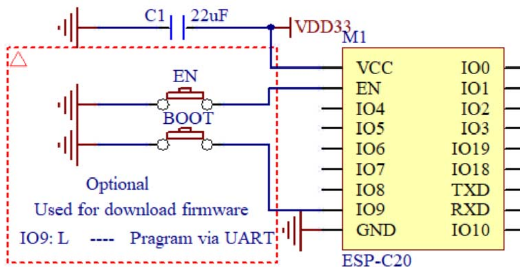
Fig.9.1 Minimum System
