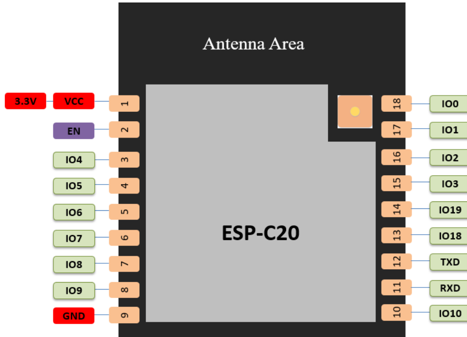
Fig.2.1 ESP-C20 Pins Definition
