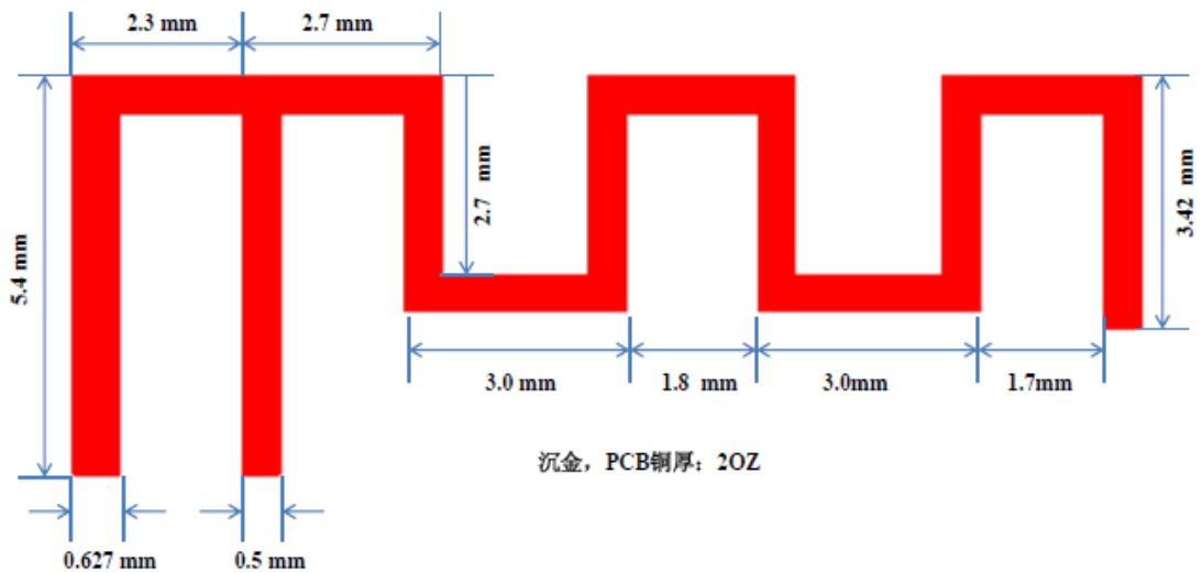
Antenna Dimension for ESP32-C3-C05
