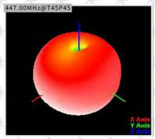
(4) Typical Free Space 3D Radiation Pattern at 447MHz:
