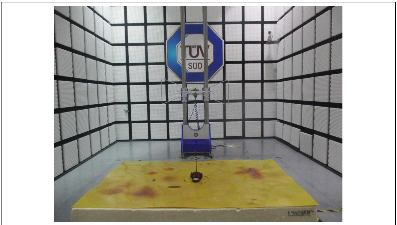
Radiated Emission test (30MHz-1GHz)
