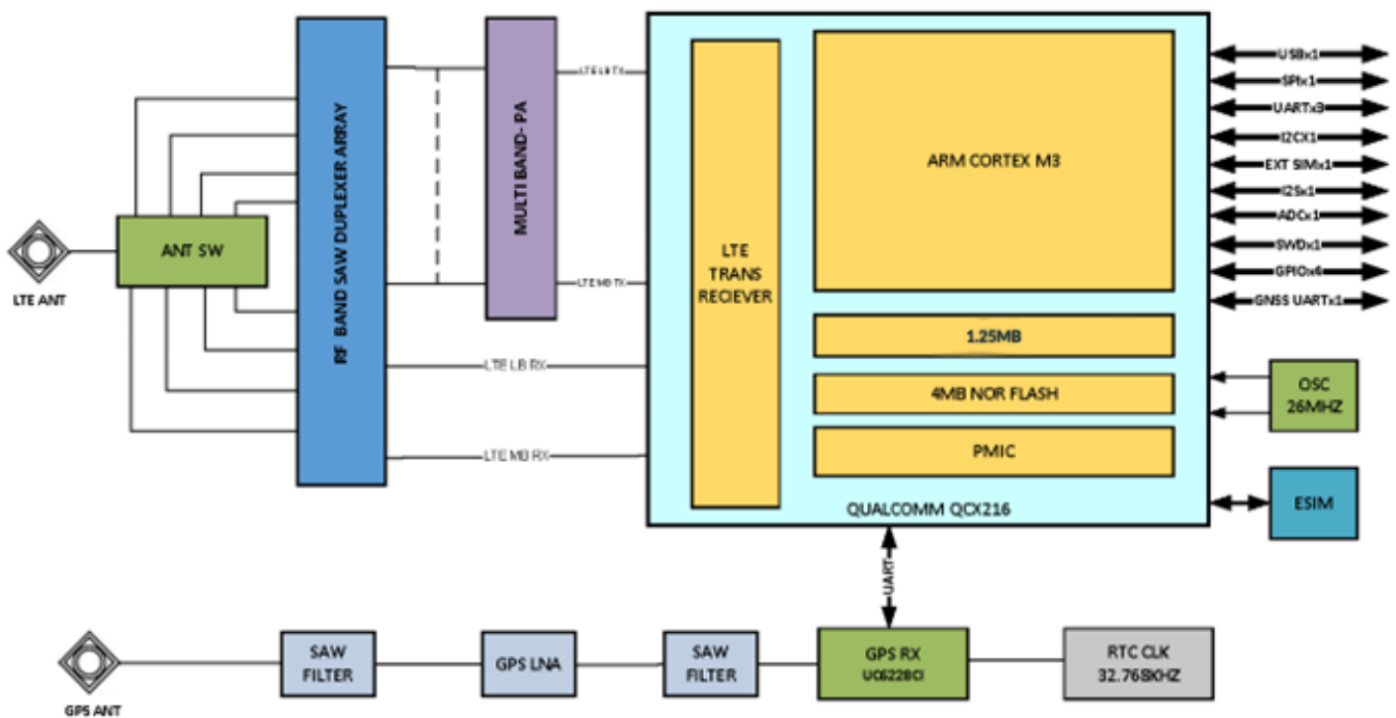
Figure 1 C16QS Functional Block Diagram
