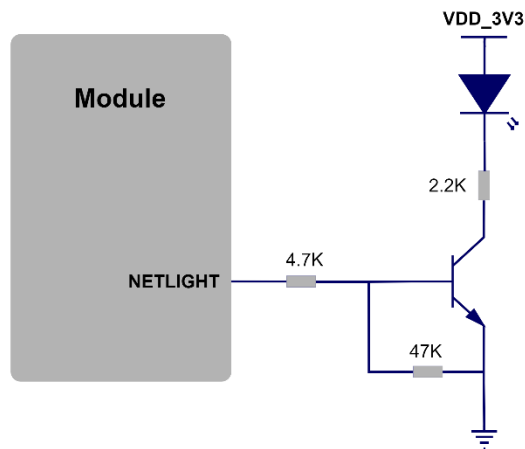
Figure 12 Net light circuit diagram
