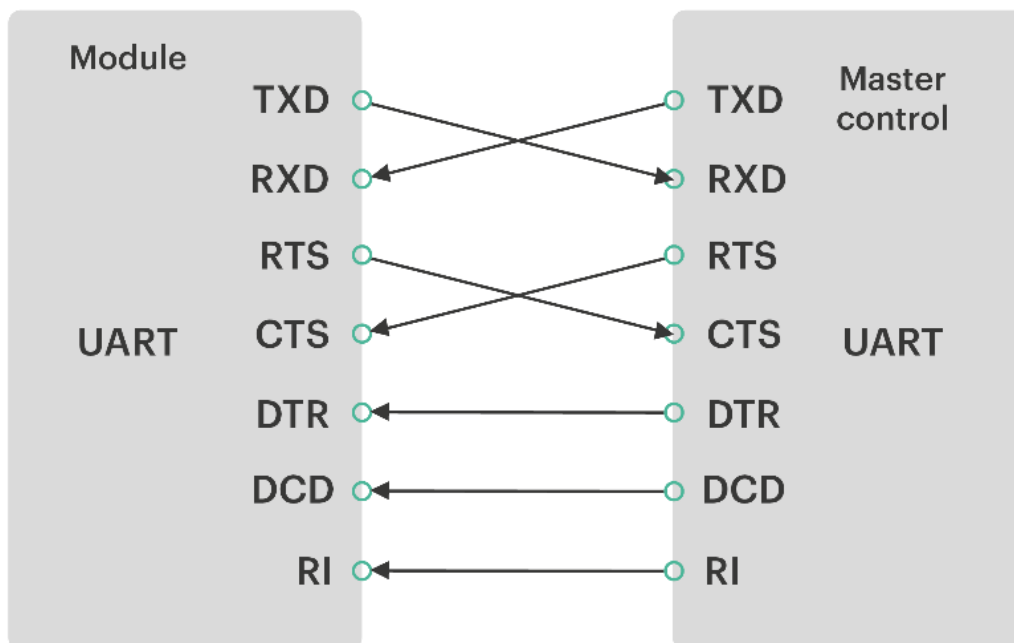
Figure 8 Full-featured serial port design
