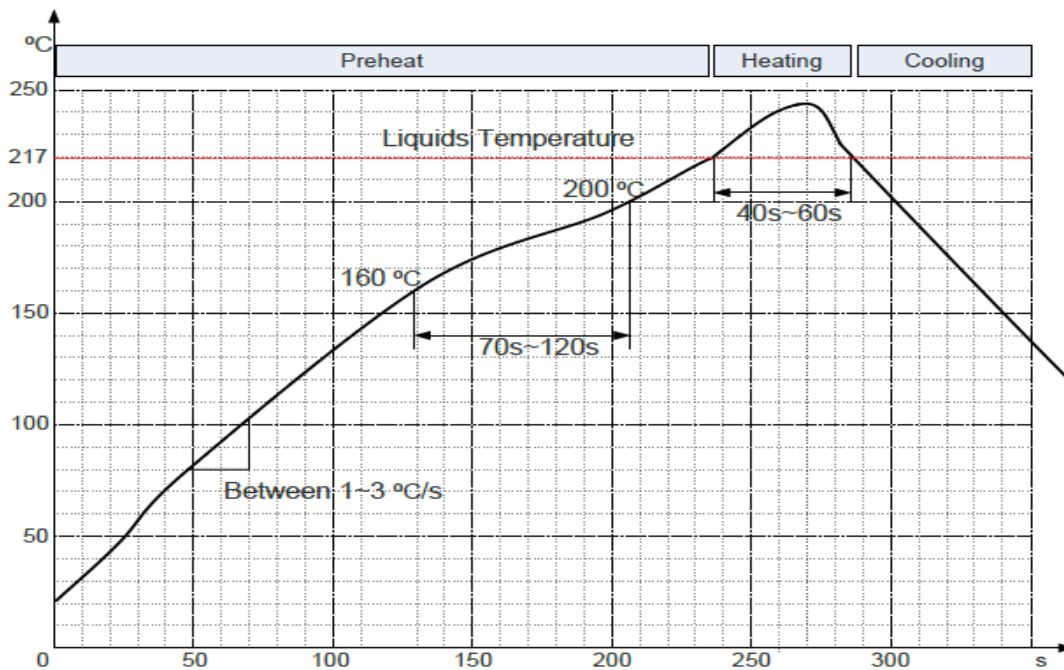
Figure 33 Reflow soldering temperature graph
