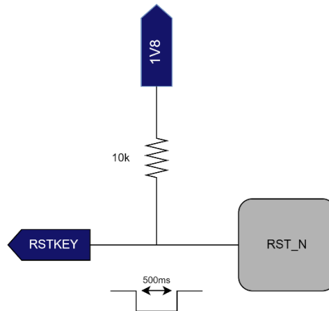
Figure 6 Reset reference circuit
