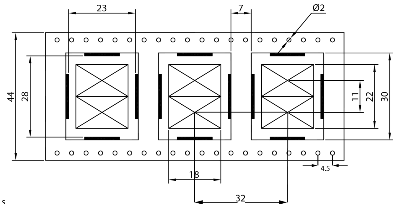
Figure 31 C16QS Tape Measurements (in mm)
