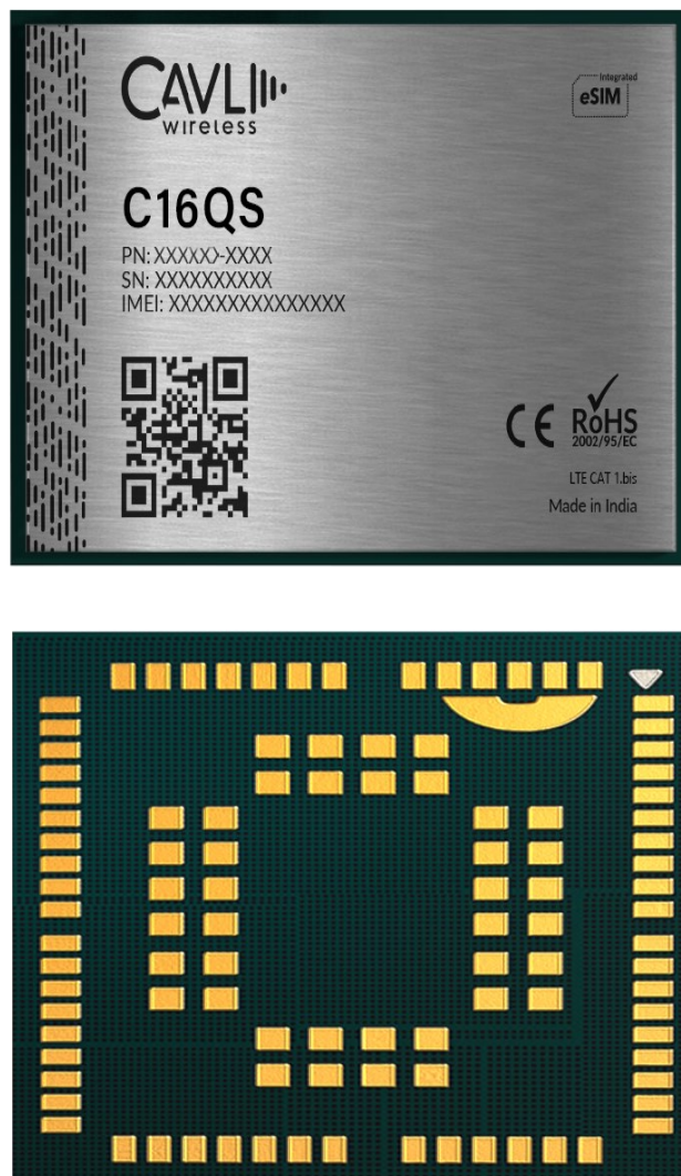
Figure 26 Top view and bottom view of the module
