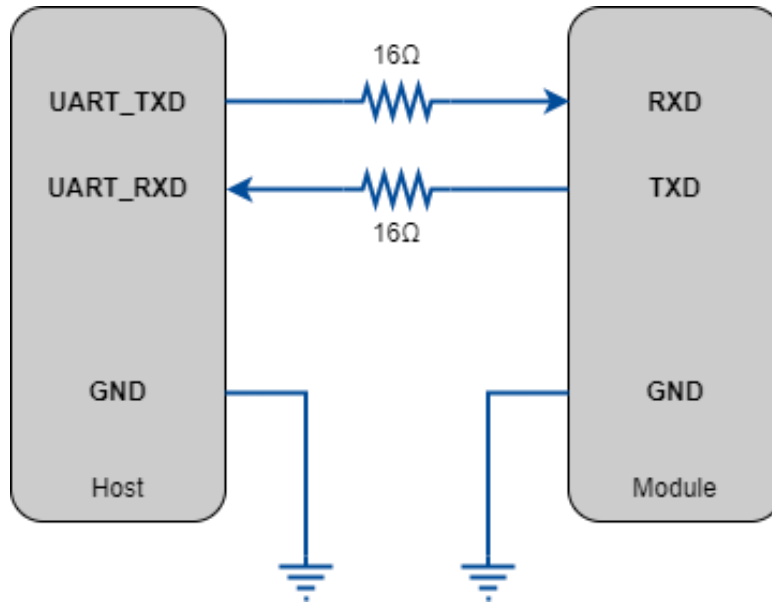
Figure 9 UART serial port design
