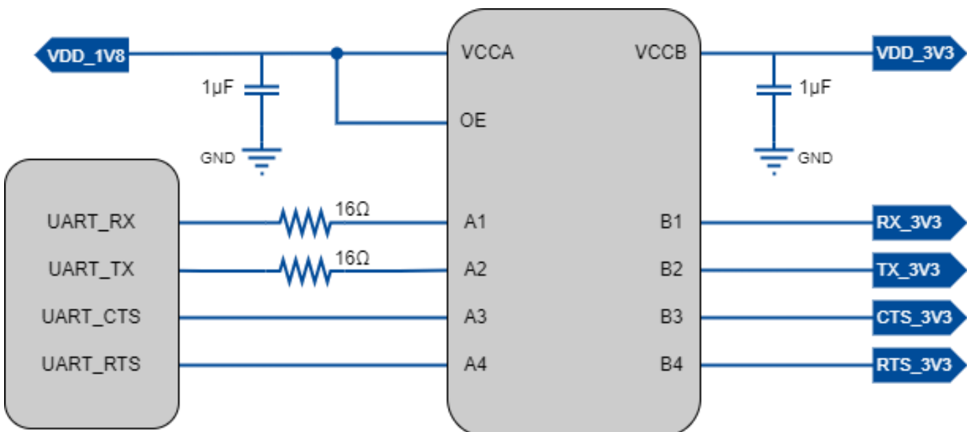
Figure 10 Level conversion chip circuit
