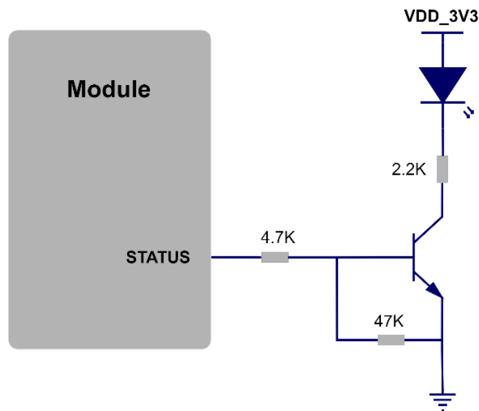
Figure 13 STATUS Pin Reference Circuit
