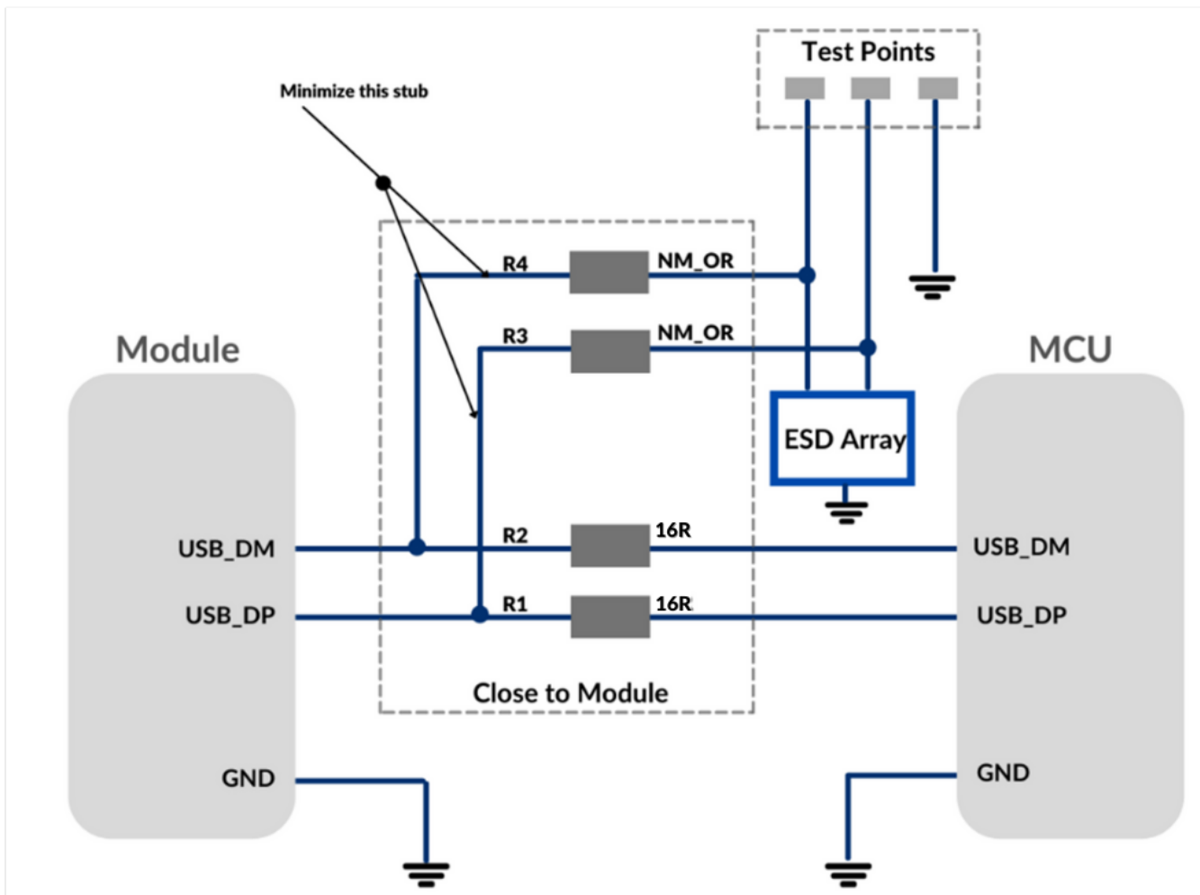
Figure 7 USB connection design circuit diagram
