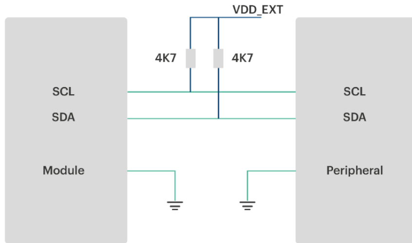
Figure 14 I2C interface reference circuit diagram
