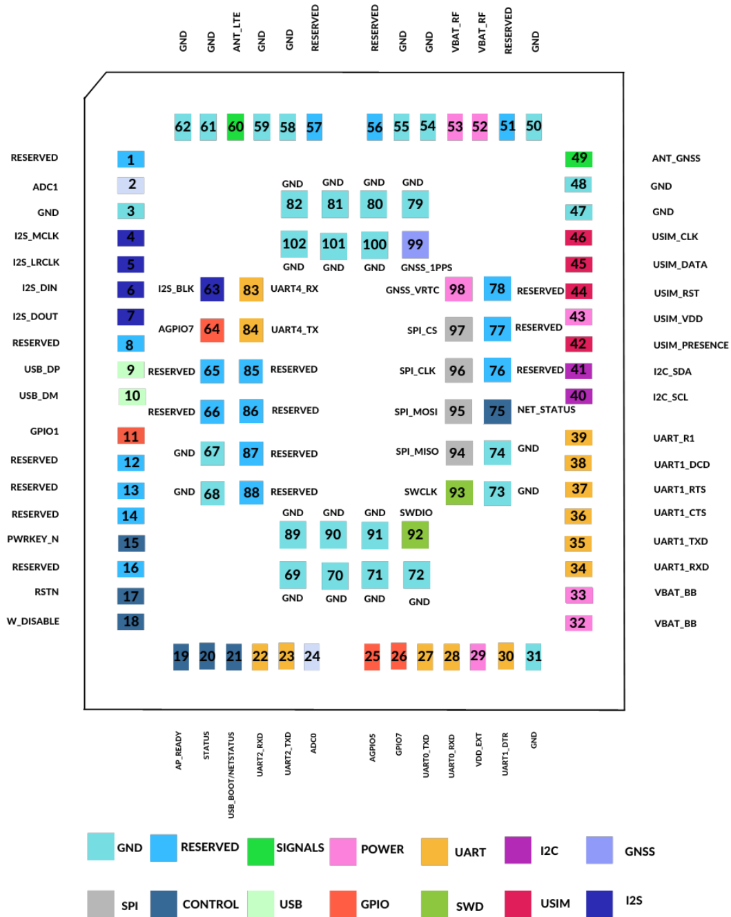
Figure 2 C16QS module Interface definition (top view)
