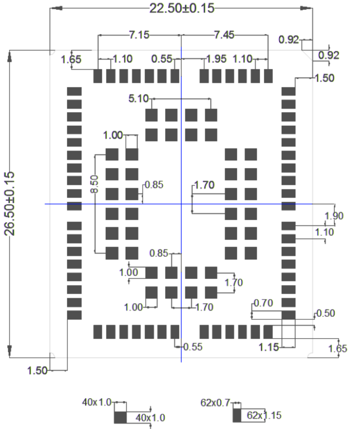
Figure 28 Bottom view of the module (unit: mm)
