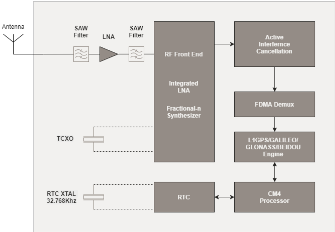
Figure 24 Multi GNSS receiver Block diagram
