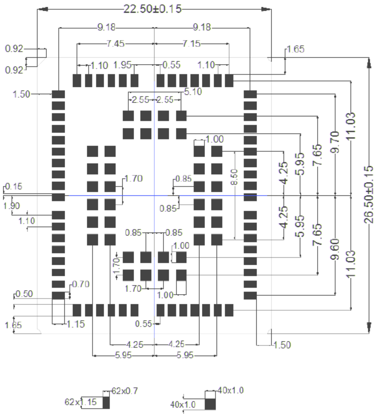
Figure 29 Recommended Footprint (Top View) (unit: mm)
