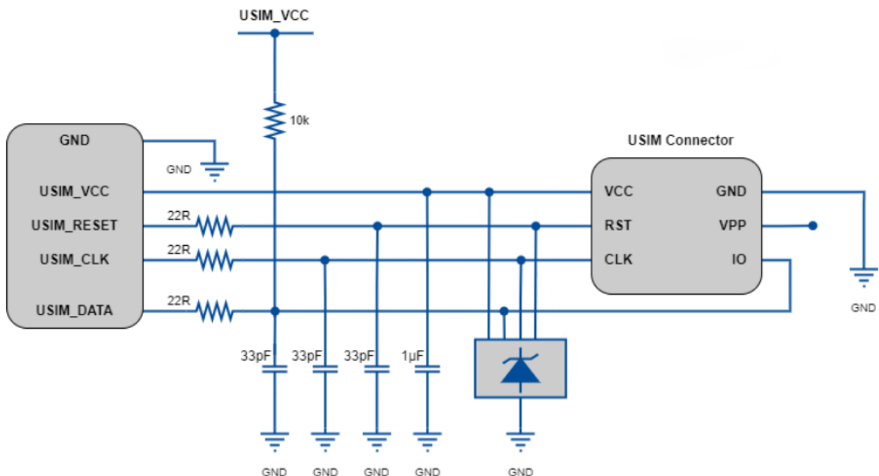
Figure 11 USIM design circuit diagram
