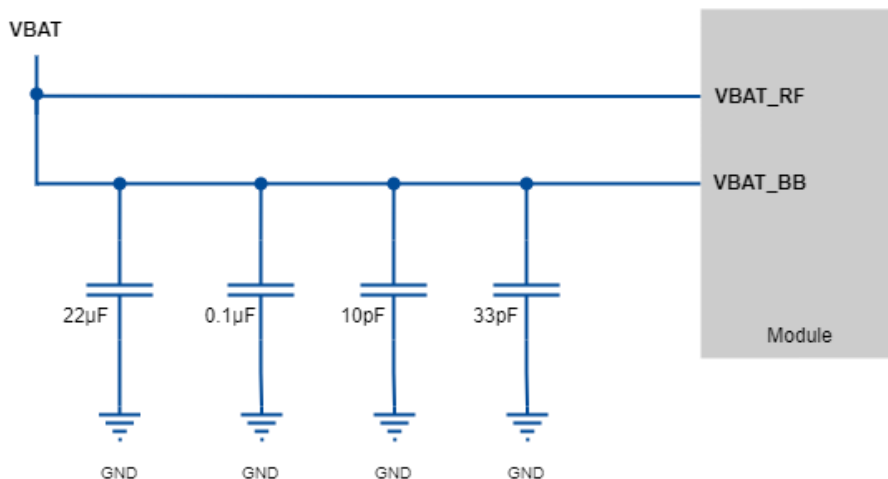
Figure 3 VBAT power supply
