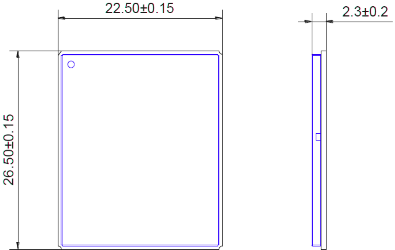
Figure 27 Front view and side view of the module (unit: mm)
