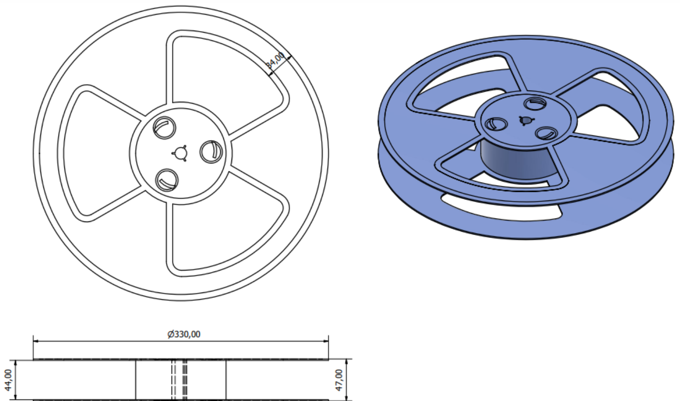
Figure 32 Reel Dimensions of C16QS (in mm)
