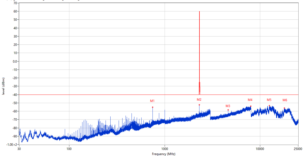
RSE (RF) _FCC PART22&24&27_LTE Band 40 _2300-2400_30MHz-25GHz - 2305-2315
