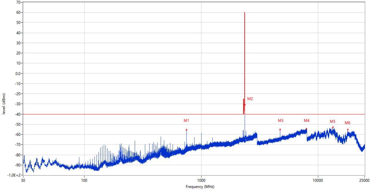
RSE (RF) _FCC PART22&24&27_LTE Band 40 _2300-2400_30MHz-25GHz - 2350-2360
