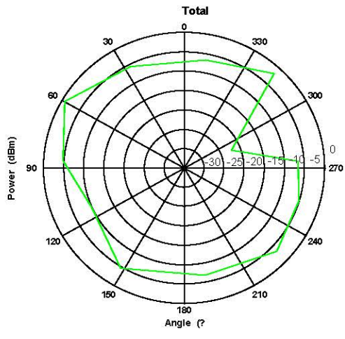
YZ Plane at f = 2.450GHz
