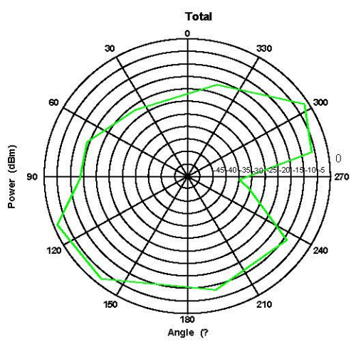
XY Plane at f = 2.450GHz
