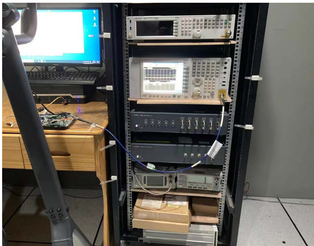
ANTENNA-PORT CONDUCTED
