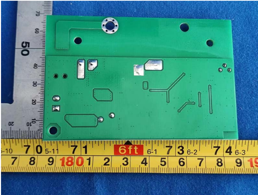
FIGURE 21 HOI CROSS+ (CT1062-400US) PANEL COVER REMOVE
