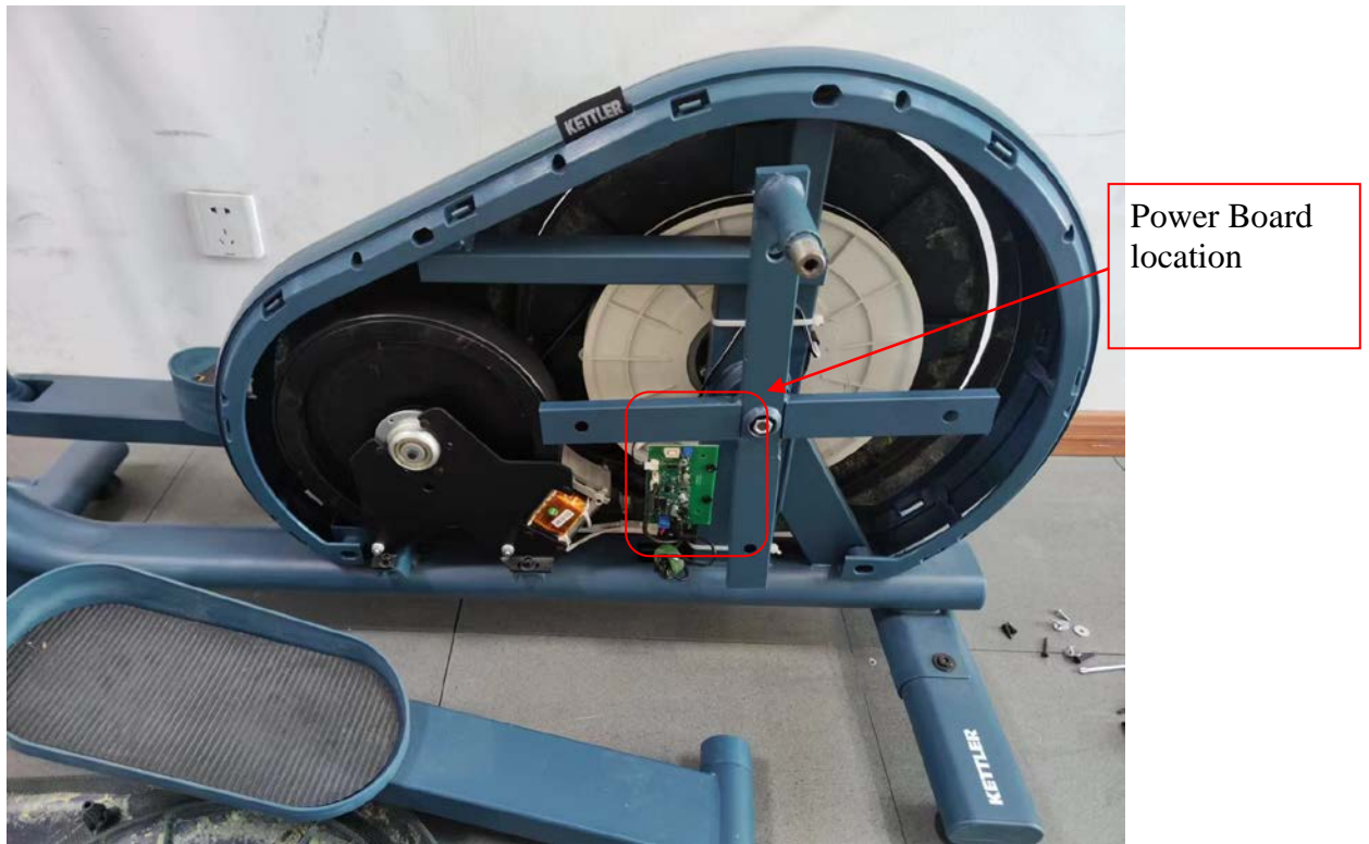
FIGURE 17 HOI CROSS+ (CT1062-400US) COVER REMOVE
