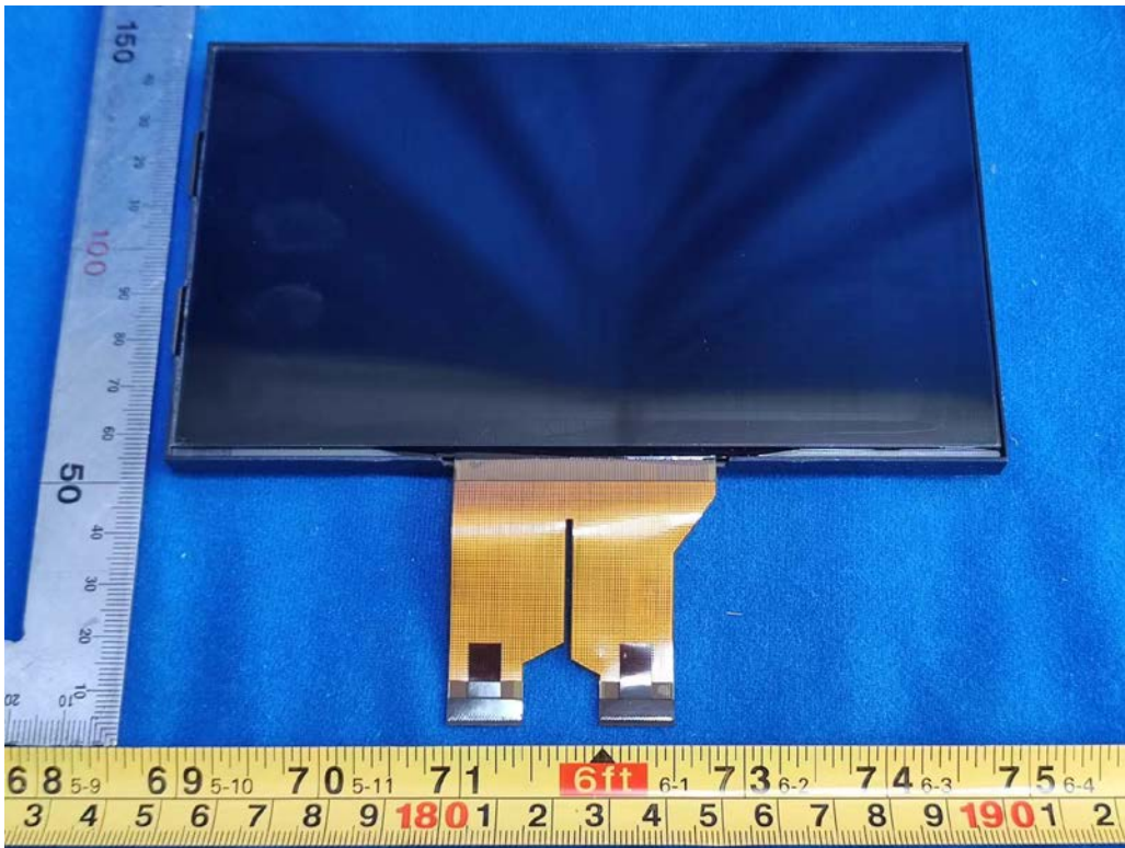
FIGURE 29 HOI CROSS+ (CT1062-400US) DISPLAY FRONT
