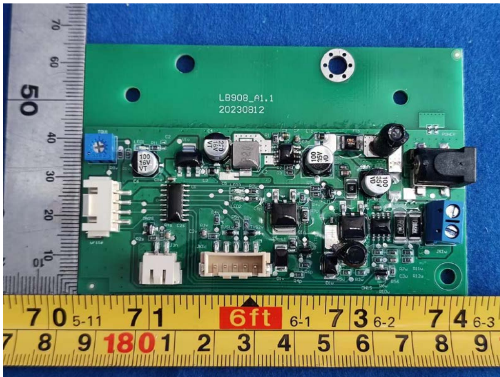
FIGURE 19 HOI CROSS+ (CT1062-400US) POWER BOARD FRONT
