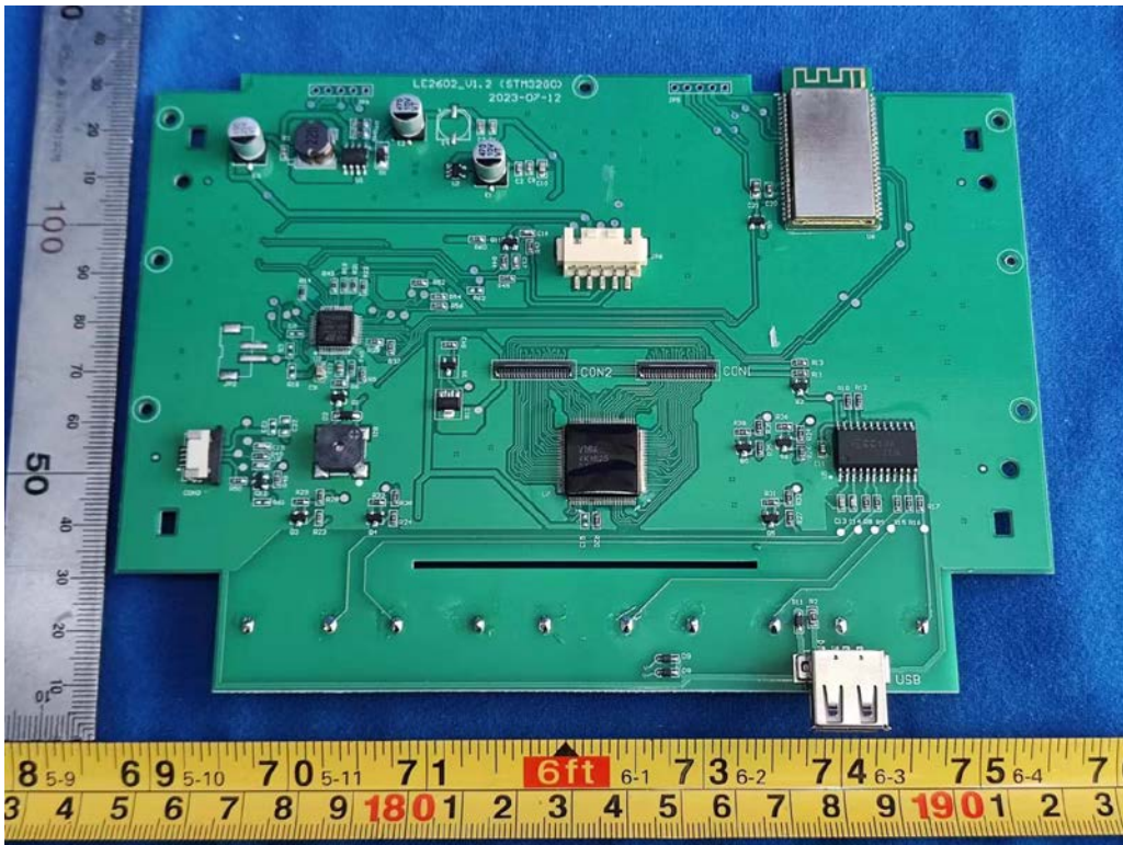
FIGURE 25 HOI CROSS+ (CT1062-400US) PANEL MAINBOARD FRONT
