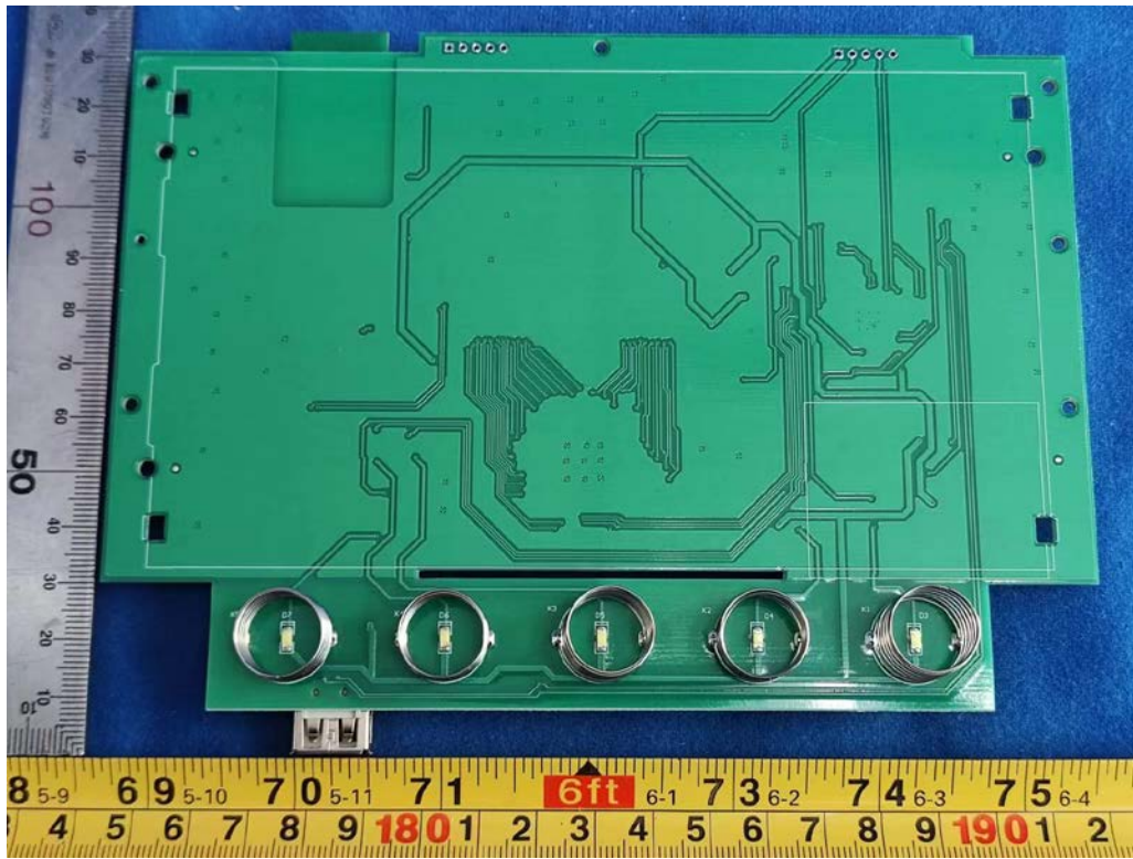
FIGURE 27 HOI CROSS+ (CT1062-400US) SHIELD REMOVE
