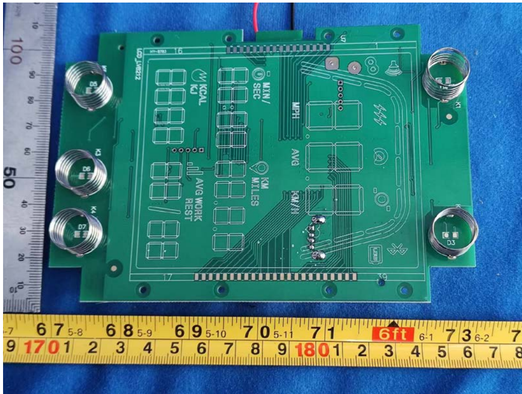
FIGURE 14 HOI CROSS (CT1061-400US) DISPLAY FRONT
