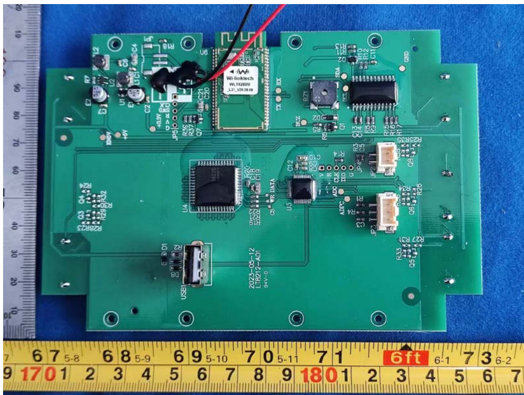
FIGURE 12 HOI CROSS (CT1061-400US) MAINBOARD FRONT
