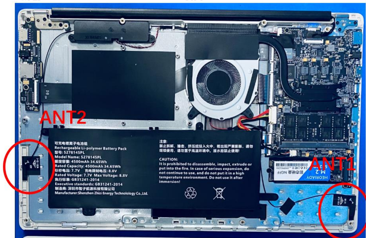
REAR VIEW
