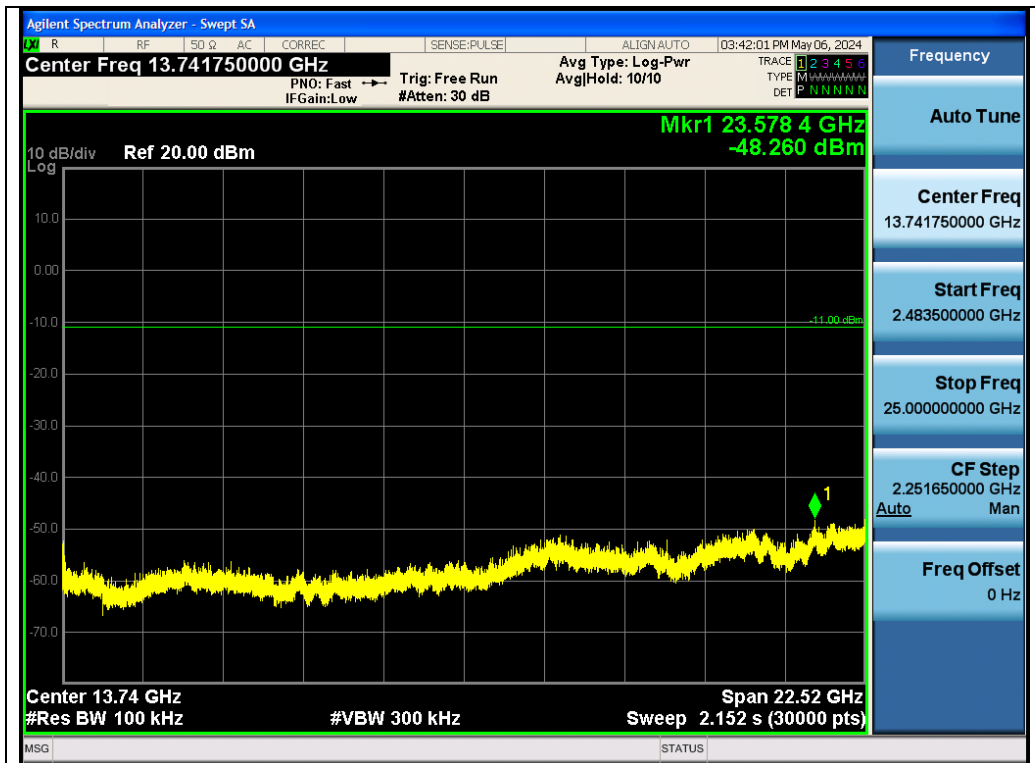
Test_Graph_2.4G_ANT1_2410_Higher Band Emissions
