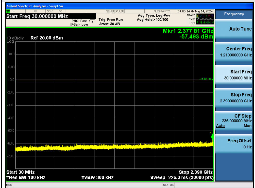
Test_Graph_2.4G_ANT1_2410_Lower Band Emissions
