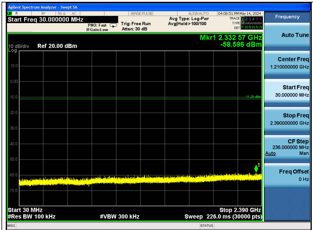
Test_Graph_2.4G_ANT1_2445_Lower Band Emissions
