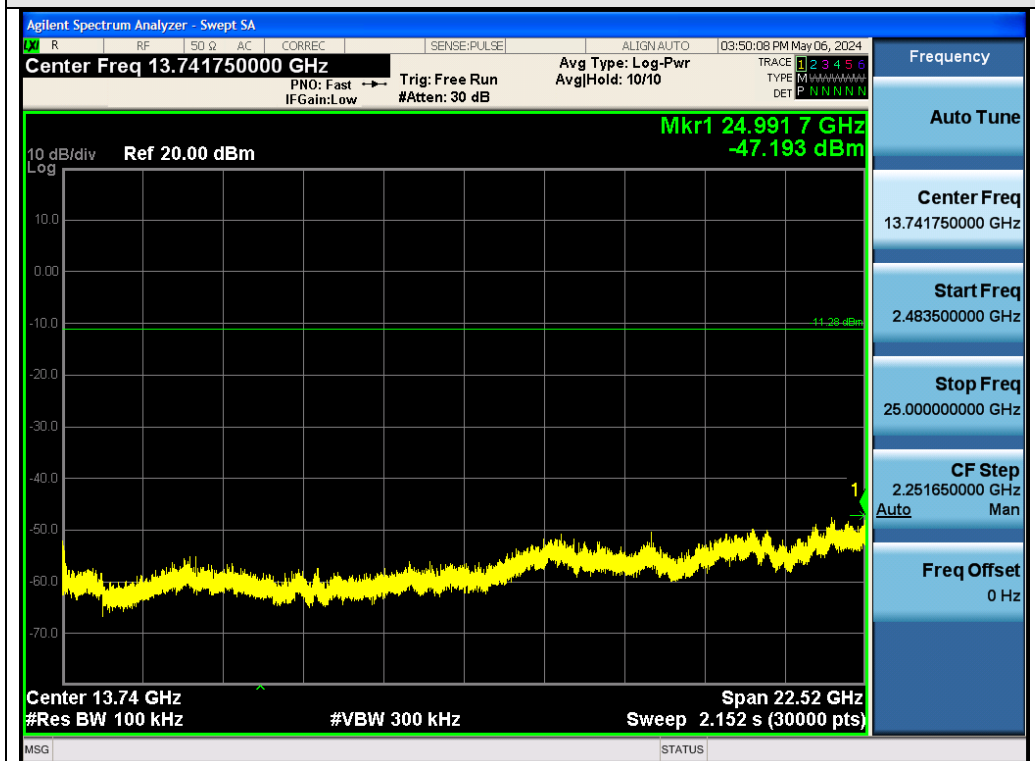
Test_Graph_2.4G_ANT1_2445_Higher Band Emissions
