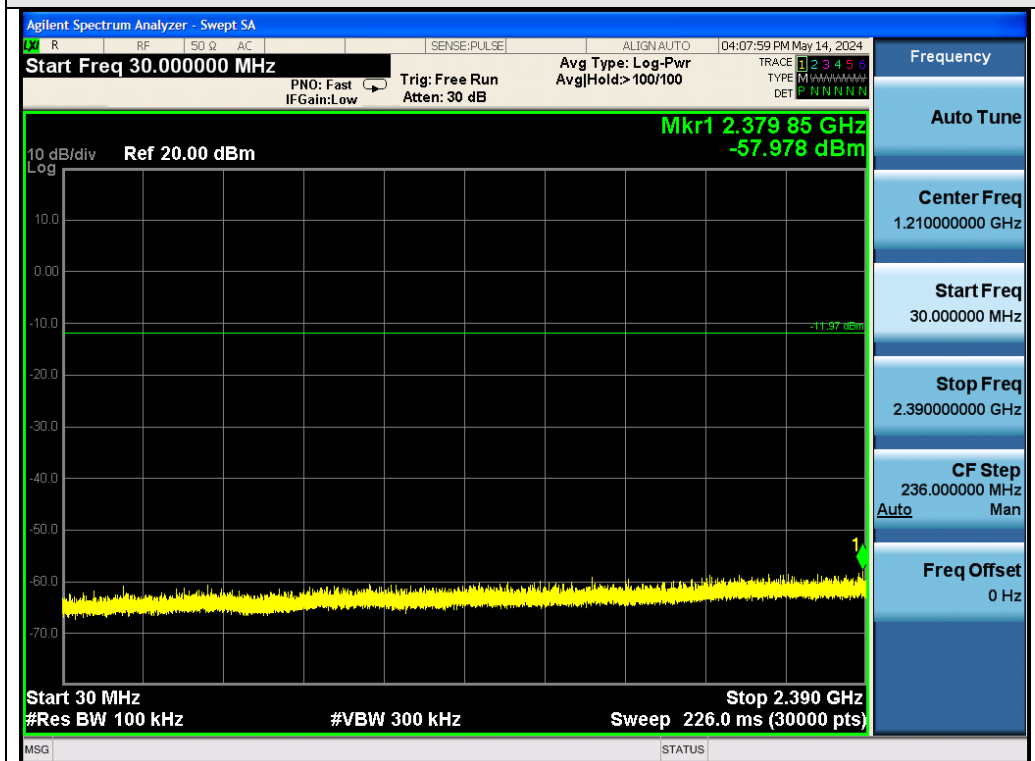
Test_Graph_2.4G_ANT1_2474_Lower Band Emissions
