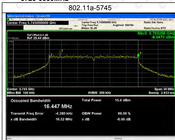
ANT1: 5725-5850MHz
