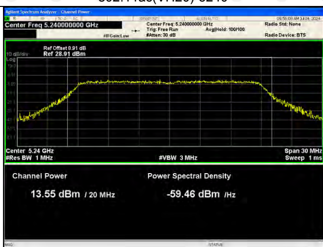
802.11ac(VH20)-5240
